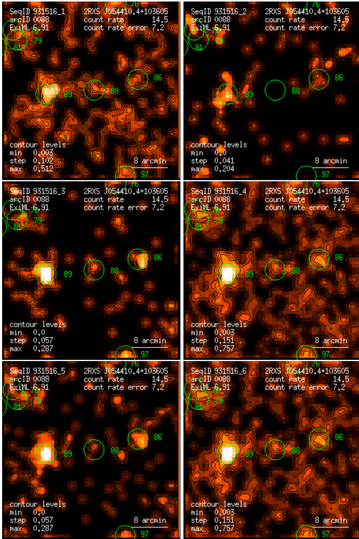
Figure 88: RASS 931516: detection 0088: band rate images, Gaussian filter: (1) PSPC channels 11 – 41, (2) 52 – 90, (3) 91 – 201, (4) 11 – 235, (5) 52 – 201, (6) 11 – 201. Broad band rates in counts/ks. Band rate contour levels in counts/ks/arcmin 2 .
