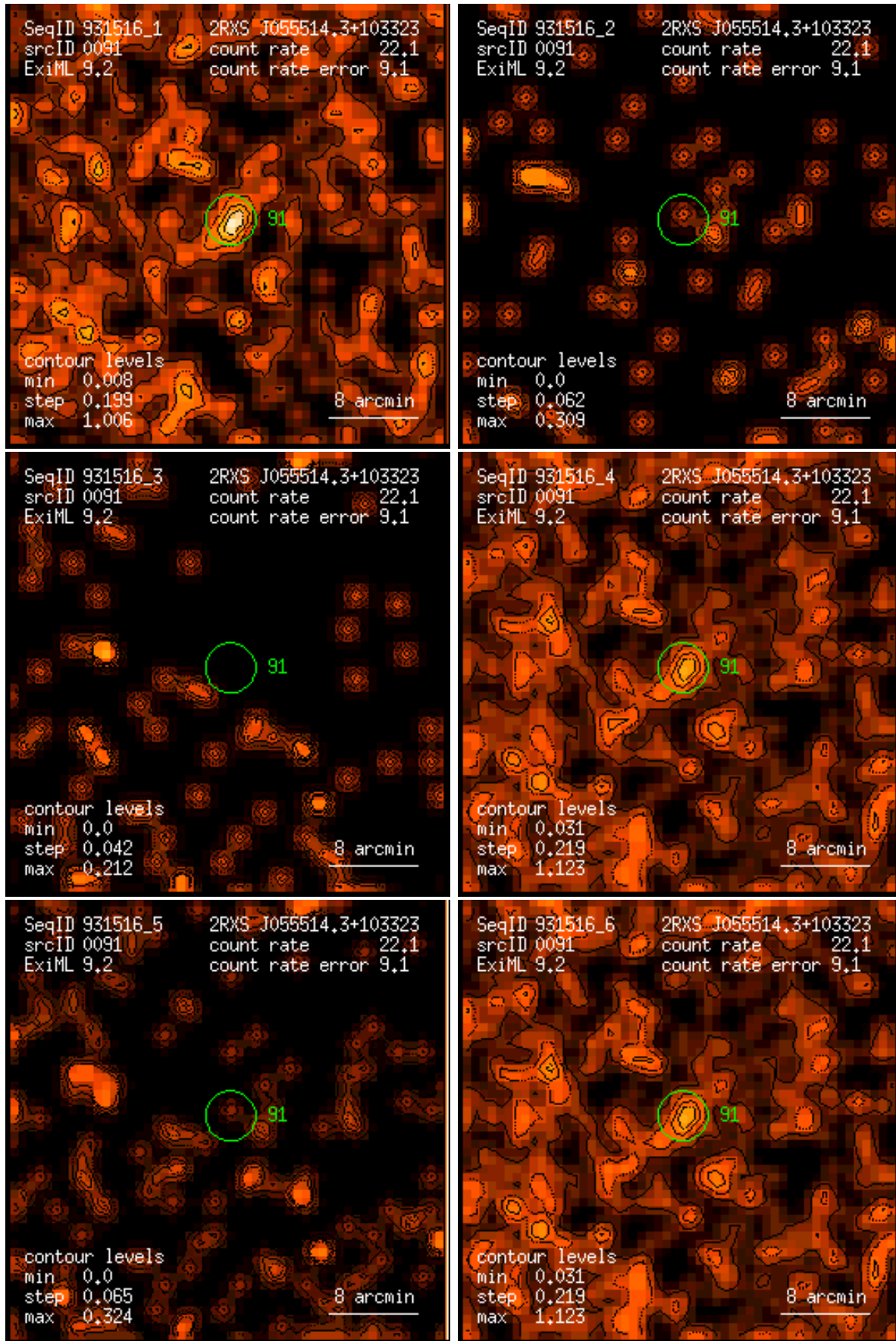
Figure 91: RASS 931516: detection 0091: band rate images, Gaussian filter: (1) PSPC channels 11 – 41, (2) 52 – 90, (3) 91 – 201, (4) 11 – 235, (5) 52 – 201, (6) 11 – 201. Broad band rates in counts/ks. Band rate contour levels in counts/ks/arcmin 2 .
