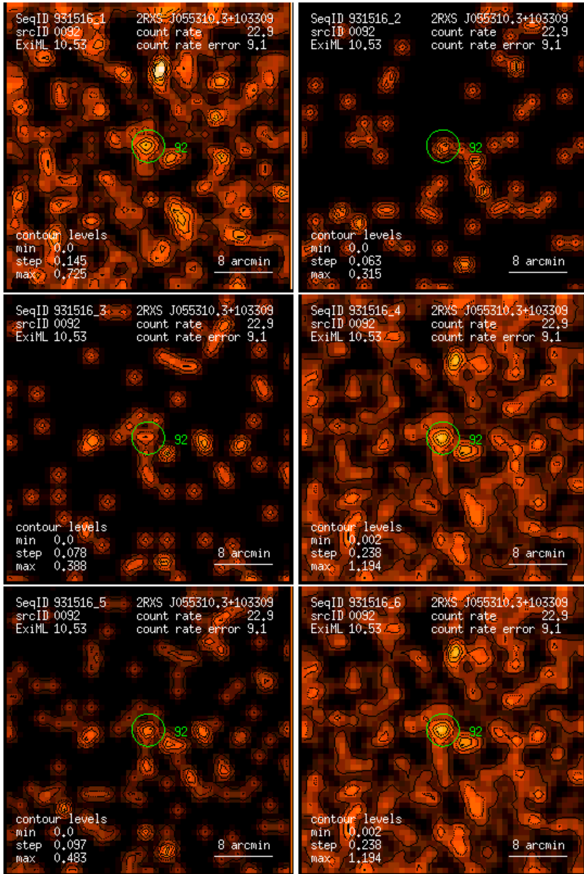
Figure 92: RASS 931516: detection 0092: band rate images, Gaussian filter: (1) PSPC channels 11 – 41, (2) 52 – 90, (3) 91 – 201, (4) 11 – 235, (5) 52 – 201, (6) 11 – 201. Broad band rates in counts/ks. Band rate contour levels in counts/ks/arcmin 2 .
