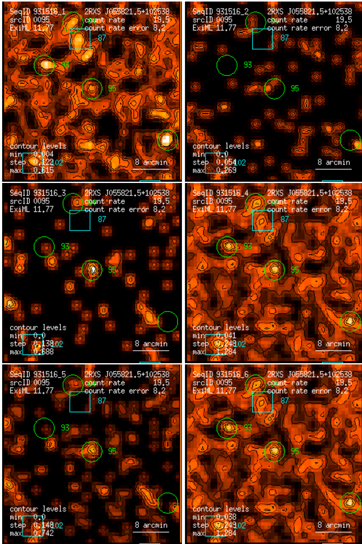
Figure 95: RASS 931516: detection 0095: band rate images, Gaussian filter: (1) PSPC channels 11 – 41, (2) 52 – 90, (3) 91 – 201, (4) 11 – 235, (5) 52 – 201, (6) 11 – 201. Broad band rates in counts/ks. Band rate contour levels in counts/ks/arcmin 2 .
