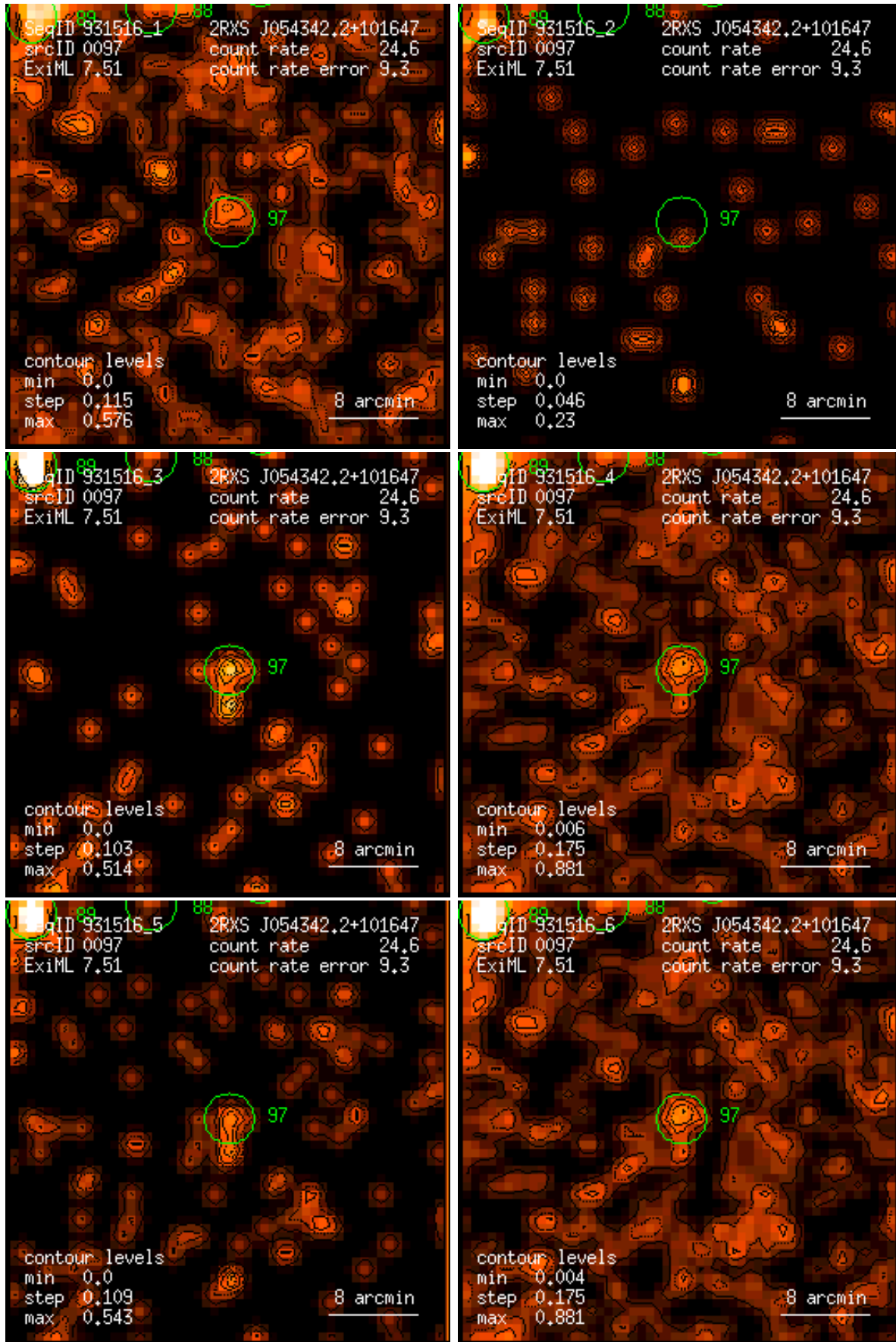
Figure 97: RASS 931516: detection 0097: band rate images, Gaussian filter: (1) PSPC channels 11 – 41, (2) 52 – 90, (3) 91 – 201, (4) 11 – 235, (5) 52 – 201, (6) 11 – 201. Broad band rates in counts/ks. Band rate contour levels in counts/ks/arcmin 2 .
