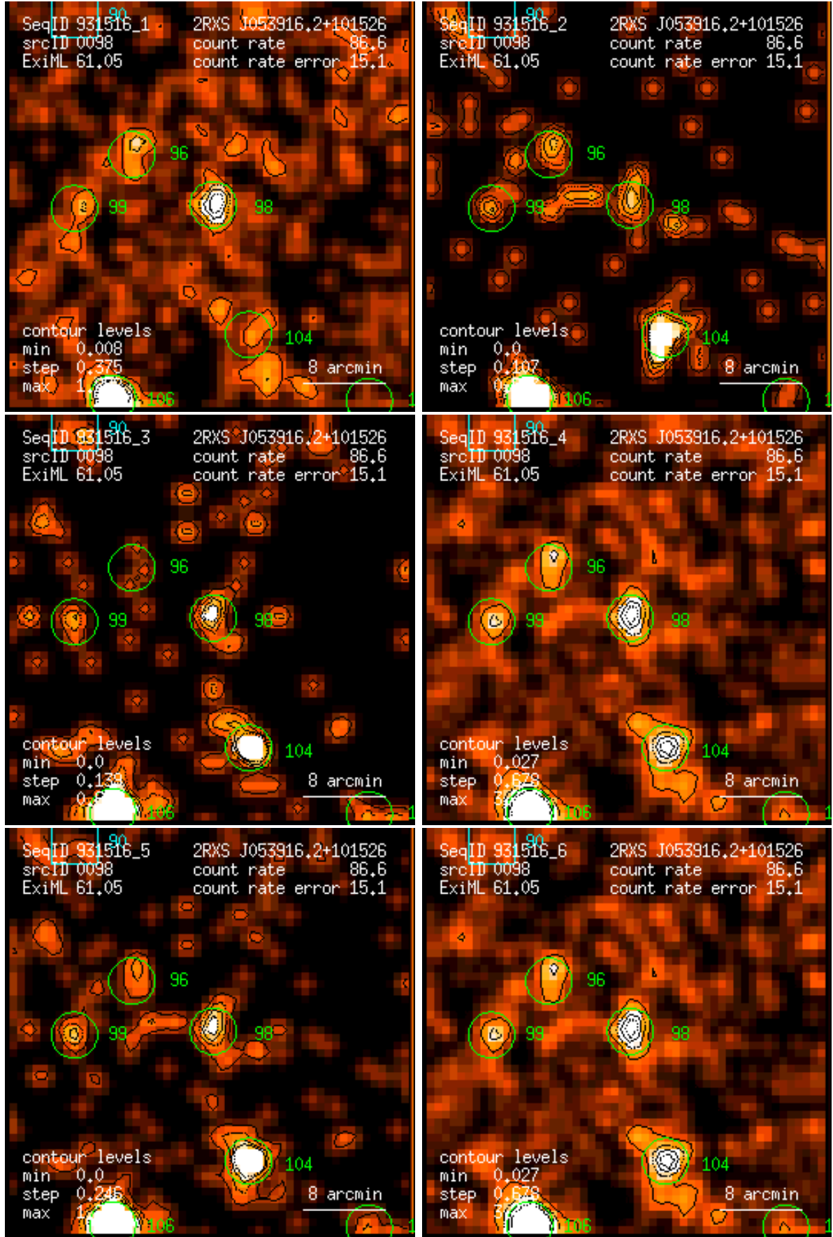
Figure 98: RASS 931516: detection 0098: band rate images, Gaussian filter: (1) PSPC channels 11 – 41, (2) 52 – 90, (3) 91 – 201, (4) 11 – 235, (5) 52 – 201, (6) 11 – 201. Broad band rates in counts/ks. Band rate contour levels in counts/ks/arcmin 2 .
