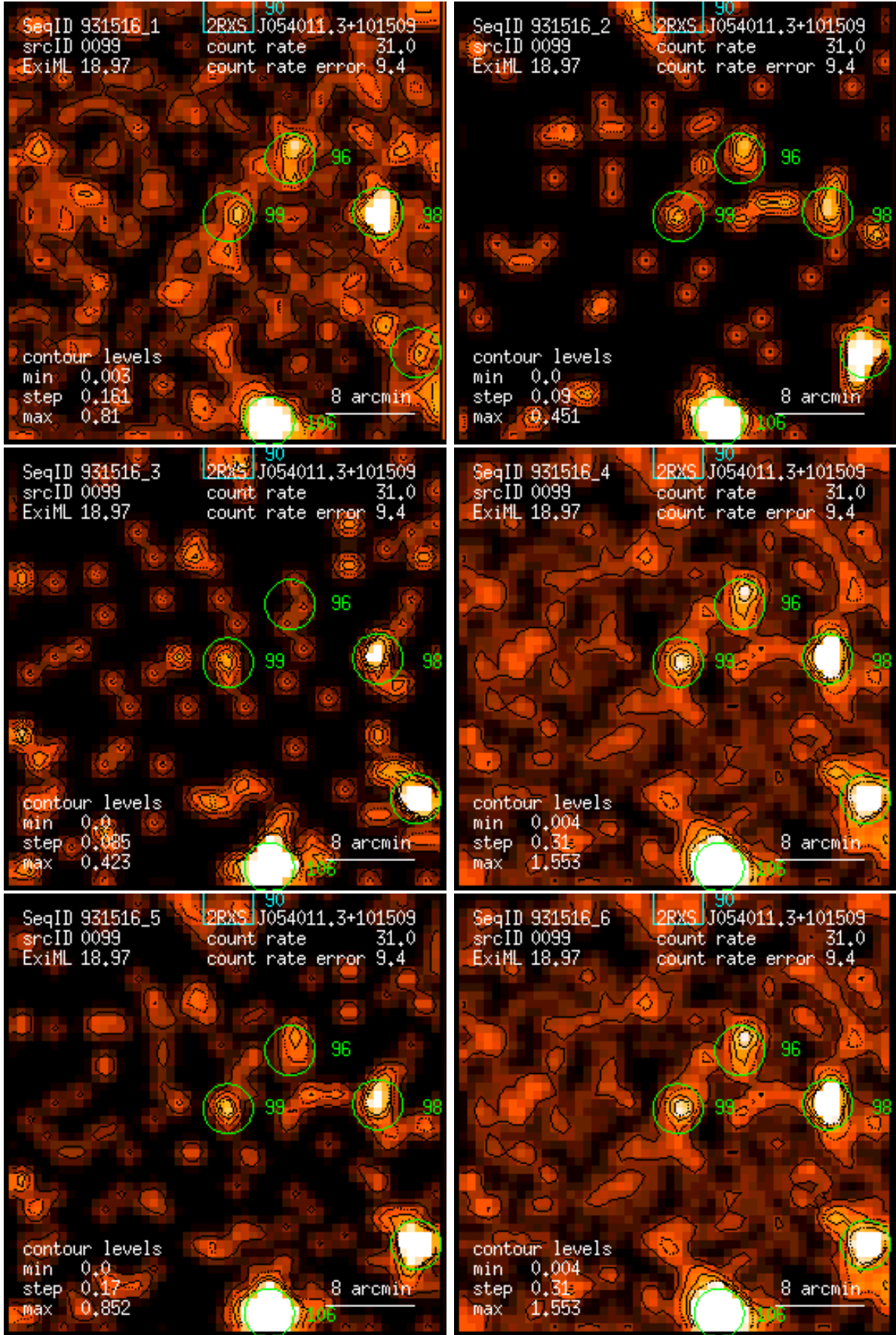
Figure 99: RASS 931516: detection 0099: band rate images, Gaussian filter: (1) PSPC channels 11 – 41, (2) 52 – 90, (3) 91 – 201, (4) 11 – 235, (5) 52 – 201, (6) 11 – 201. Broad band rates in counts/ks. Band rate contour levels in counts/ks/arcmin 2 .
