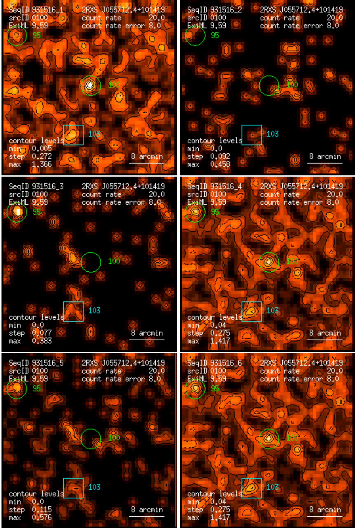
Figure 100: RASS 931516: detection 0100: band rate images, Gaussian filter: (1) PSPC channels 11 – 41, (2) 52 – 90, (3) 91 – 201, (4) 11 – 235, (5) 52 – 201, (6) 11 – 201. Broad band rates in counts/ks. Band rate contour levels in counts/ks/arcmin 2 .
