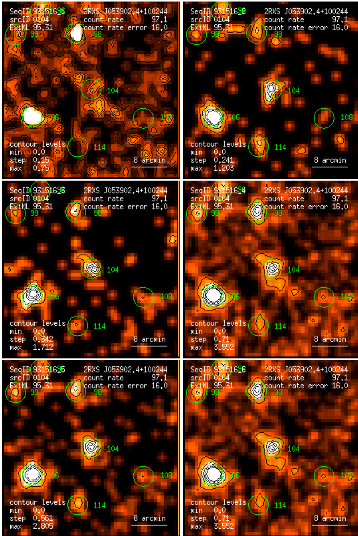
Figure 104: RASS 931516: detection 0104: band rate images, Gaussian filter: (1) PSPC channels 11 – 41, (2) 52 – 90, (3) 91 – 201, (4) 11 – 235, (5) 52 – 201, (6) 11 – 201. Broad band rates in counts/ks. Band rate contour levels in counts/ks/arcmin 2 .
