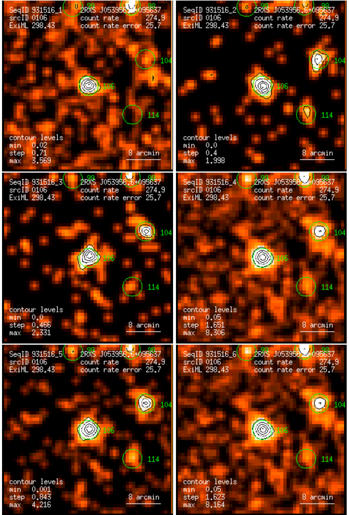
Figure 106: RASS 931516: detection 0106: band rate images, Gaussian filter: (1) PSPC channels 11 – 41, (2) 52 – 90, (3) 91 – 201, (4) 11 – 235, (5) 52 – 201, (6) 11 – 201. Broad band rates in counts/ks. Band rate contour levels in counts/ks/arcmin 2 .
