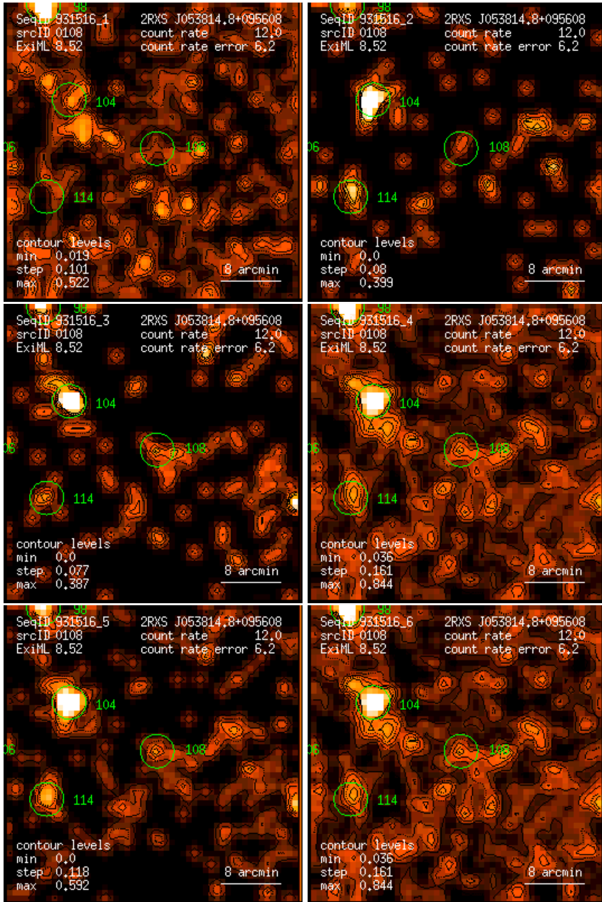
Figure 108: RASS 931516: detection 0108: band rate images, Gaussian filter: (1) PSPC channels 11 – 41, (2) 52 – 90, (3) 91 – 201, (4) 11 – 235, (5) 52 – 201, (6) 11 – 201. Broad band rates in counts/ks. Band rate contour levels in counts/ks/arcmin 2 .
