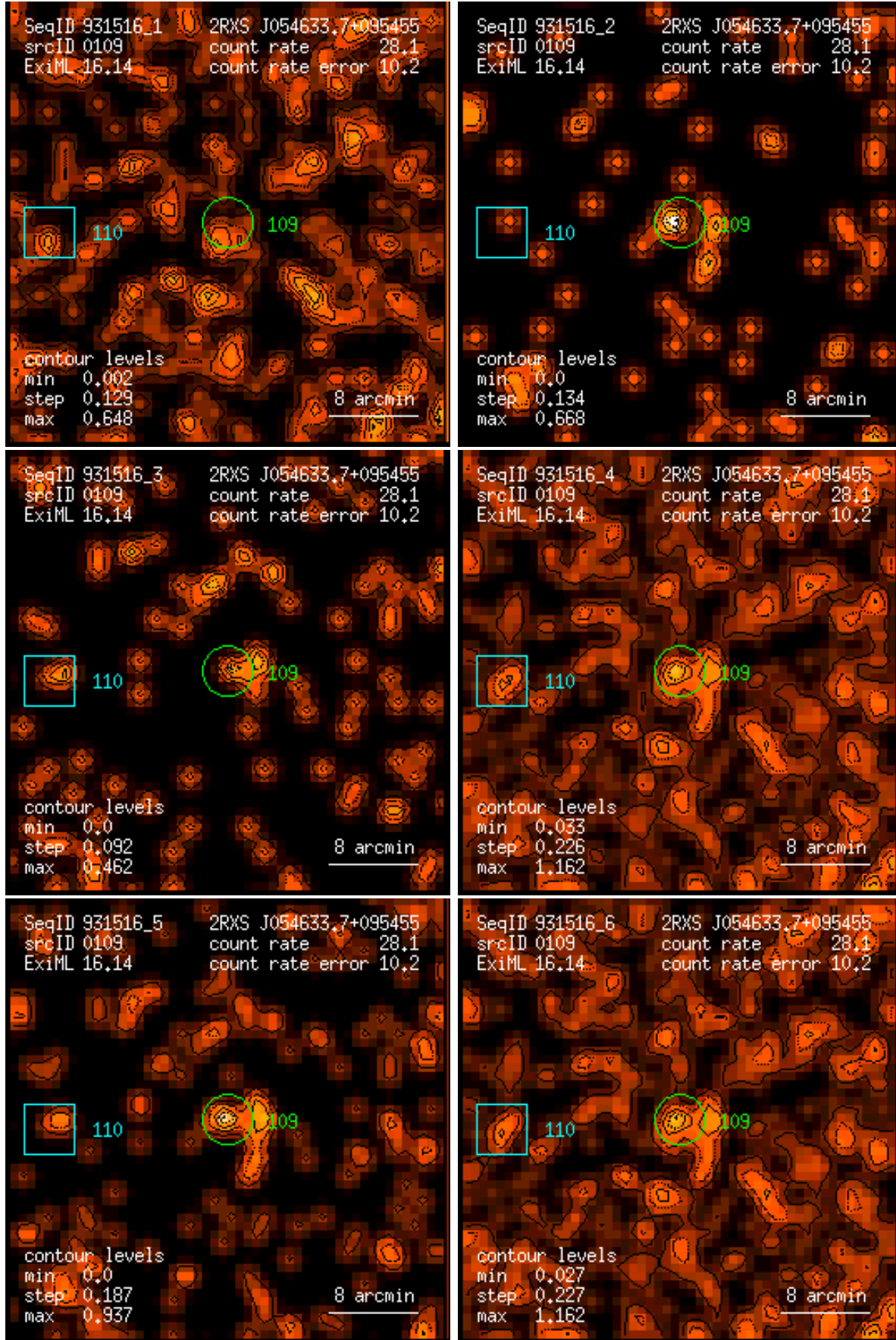
Figure 109: RASS 931516: detection 0109: band rate images, Gaussian filter: (1) PSPC channels 11 – 41, (2) 52 – 90, (3) 91 – 201, (4) 11 – 235, (5) 52 – 201, (6) 11 – 201. Broad band rates in counts/ks. Band rate contour levels in counts/ks/arcmin 2 .
