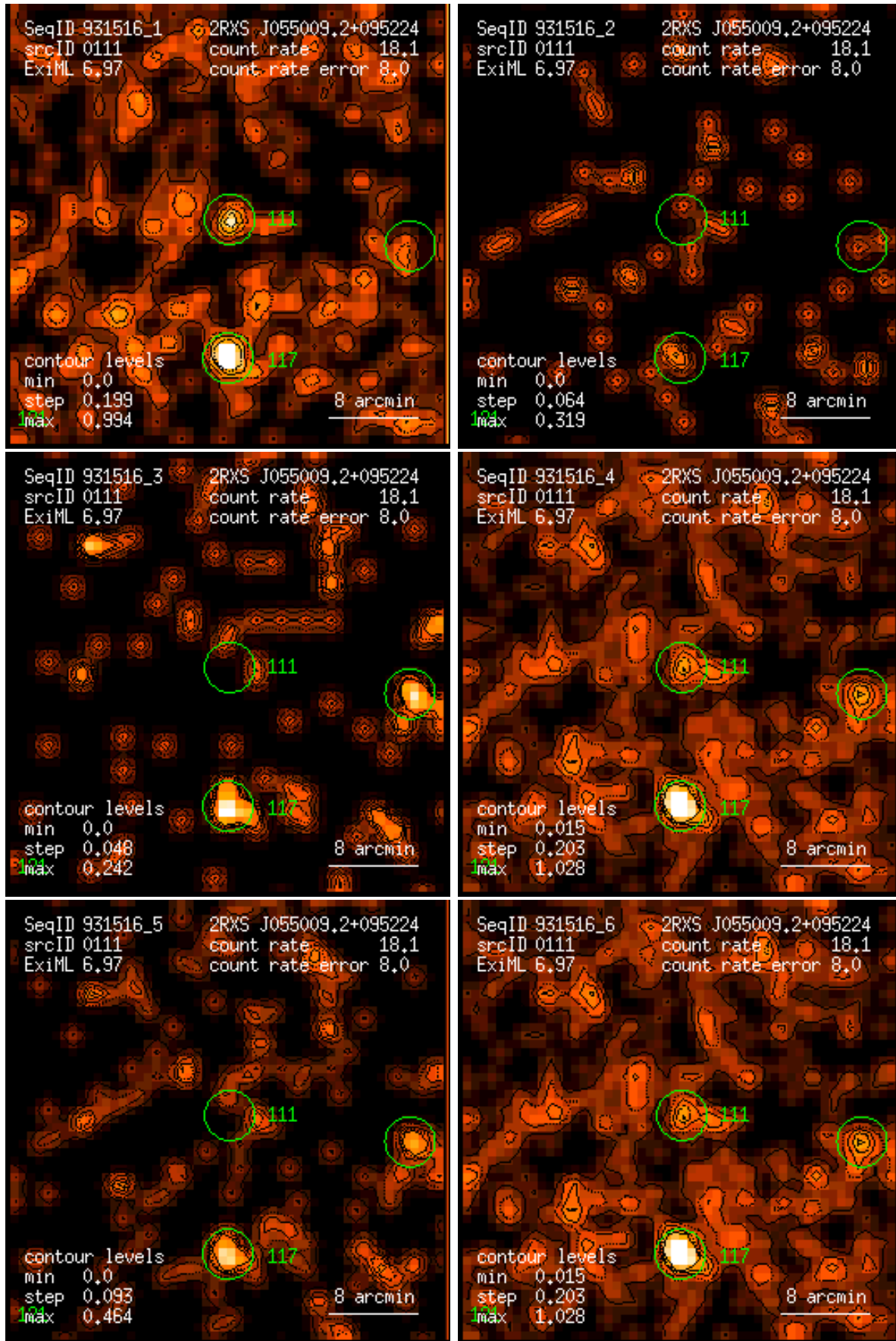
Figure 111: RASS 931516: detection 0111: band rate images, Gaussian filter: (1) PSPC channels 11 – 41, (2) 52 – 90, (3) 91 – 201, (4) 11 – 235, (5) 52 – 201, (6) 11 – 201. Broad band rates in counts/ks. Band rate contour levels in counts/ks/arcmin 2 .
