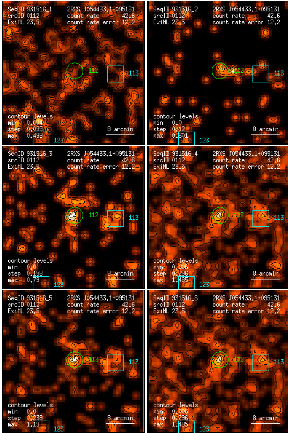
Figure 112: RASS 931516: detection 0112: band rate images, Gaussian filter: (1) PSPC channels 11 – 41, (2) 52 – 90, (3) 91 – 201, (4) 11 – 235, (5) 52 – 201, (6) 11 – 201. Broad band rates in counts/ks. Band rate contour levels in counts/ks/arcmin 2 .
