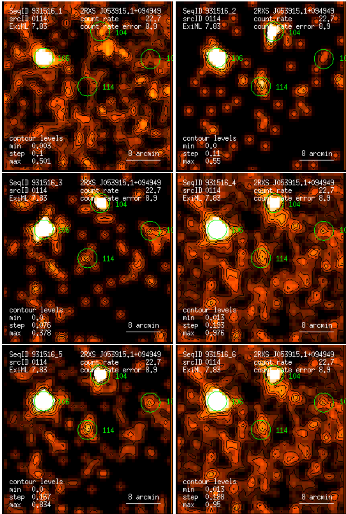
Figure 114: RASS 931516: detection 0114: band rate images, Gaussian filter: (1) PSPC channels 11 – 41, (2) 52 – 90, (3) 91 – 201, (4) 11 – 235, (5) 52 – 201, (6) 11 – 201. Broad band rates in counts/ks. Band rate contour levels in counts/ks/arcmin 2 .
