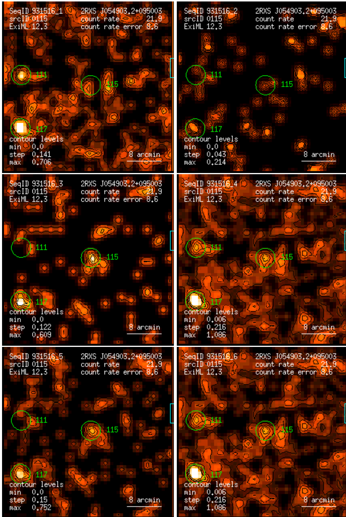
Figure 115: RASS 931516: detection 0115: band rate images, Gaussian filter: (1) PSPC channels 11 – 41, (2) 52 – 90, (3) 91 – 201, (4) 11 – 235, (5) 52 – 201, (6) 11 – 201. Broad band rates in counts/ks. Band rate contour levels in counts/ks/arcmin 2 .
