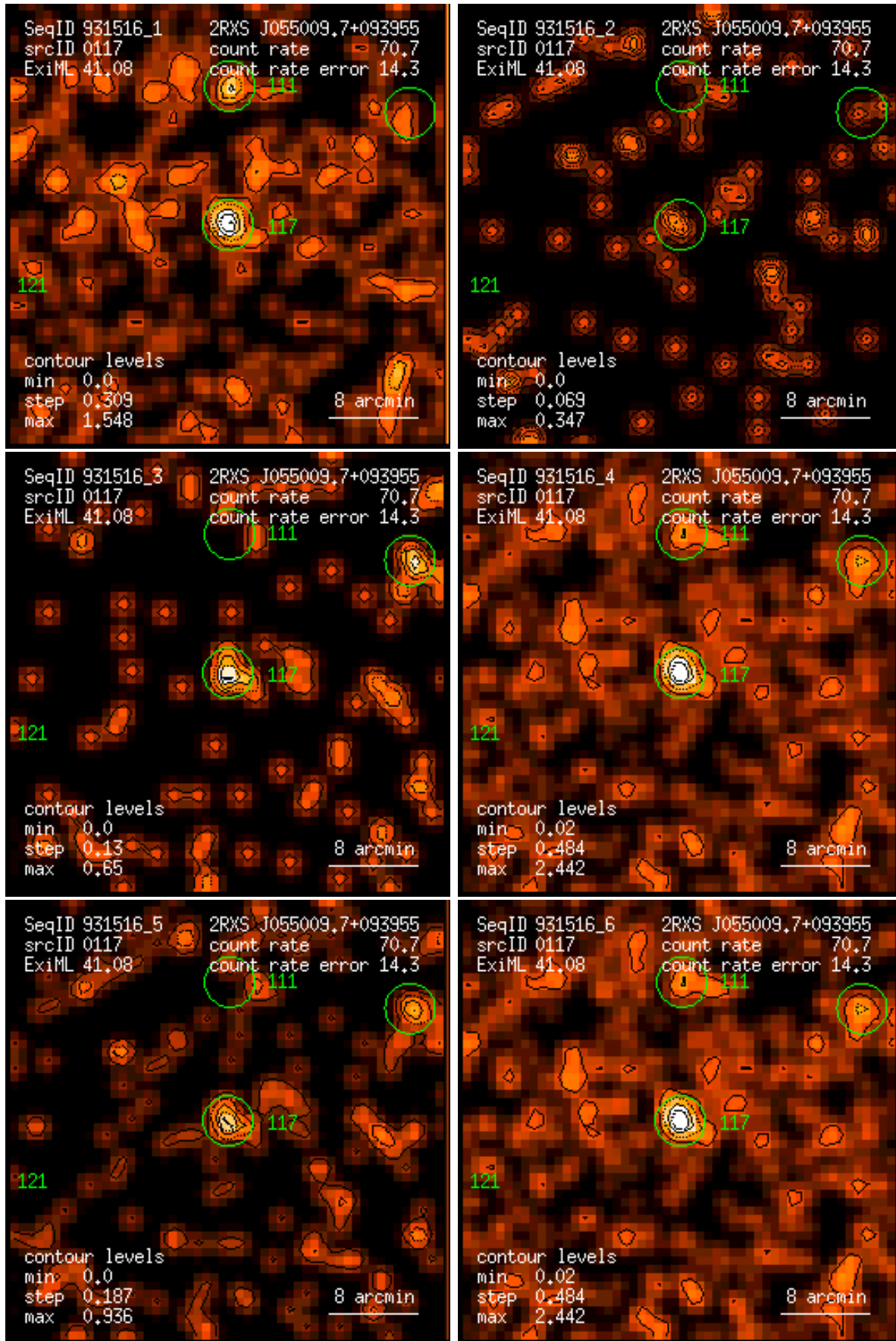
Figure 117: RASS 931516: detection 0117: band rate images, Gaussian filter: (1) PSPC channels 11 – 41, (2) 52 – 90, (3) 91 – 201, (4) 11 – 235, (5) 52 – 201, (6) 11 – 201. Broad band rates in counts/ks. Band rate contour levels in counts/ks/arcmin 2 .
