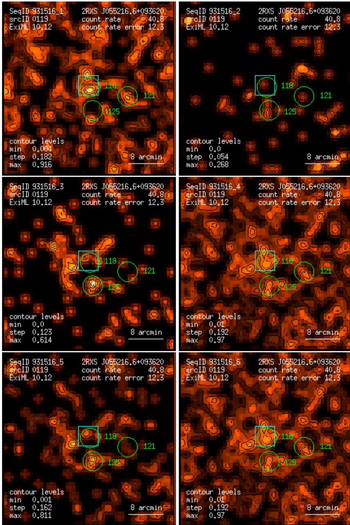
Figure 119: RASS 931516: detection 0119: band rate images, Gaussian filter: (1) PSPC channels 11 – 41, (2) 52 – 90, (3) 91 – 201, (4) 11 – 235, (5) 52 – 201, (6) 11 – 201. Broad band rates in counts/ks. Band rate contour levels in counts/ks/arcmin 2 .
