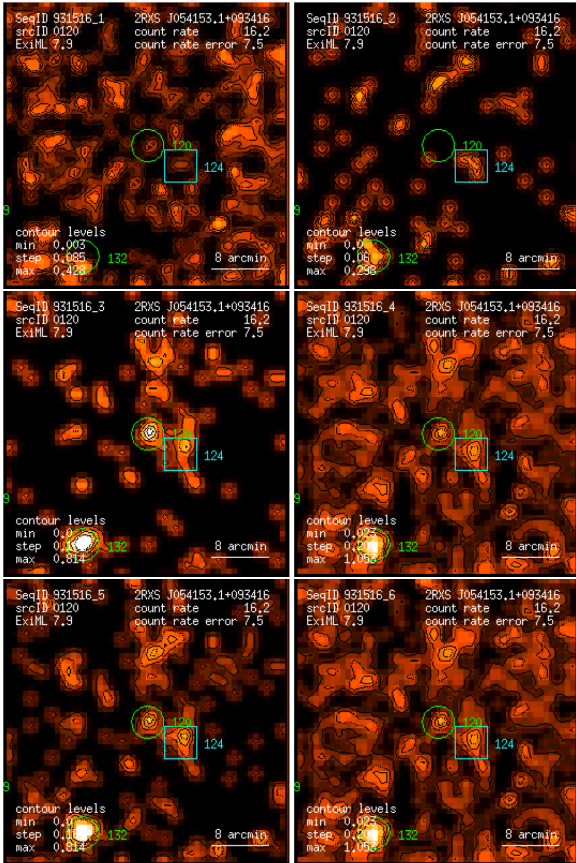
Figure 120: RASS 931516: detection 0120: band rate images, Gaussian filter: (1) PSPC channels 11 – 41, (2) 52 – 90, (3) 91 – 201, (4) 11 – 235, (5) 52 – 201, (6) 11 – 201. Broad band rates in counts/ks. Band rate contour levels in counts/ks/arcmin 2 .
