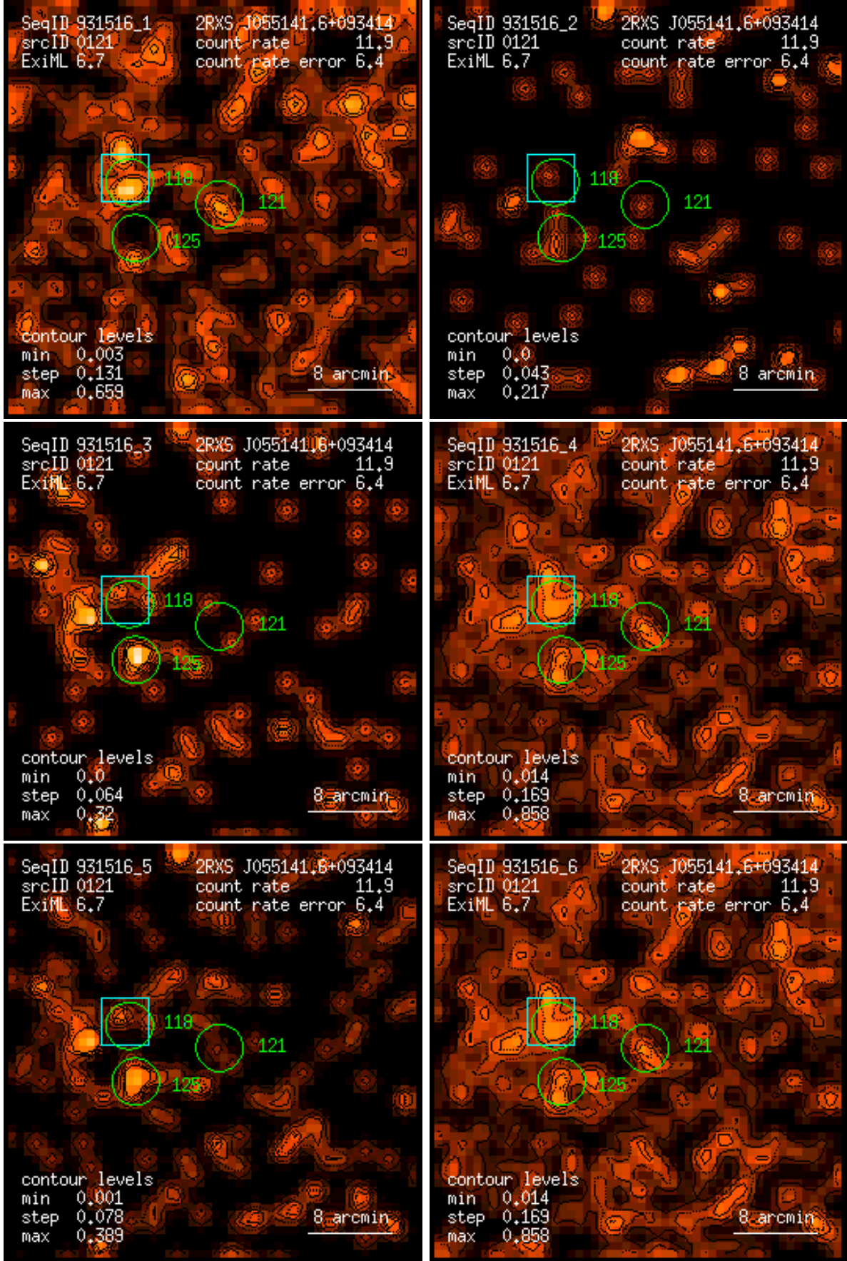
Figure 121: RASS 931516: detection 0121: band rate images, Gaussian filter: (1) PSPC channels 11 – 41, (2) 52 – 90, (3) 91 – 201, (4) 11 – 235, (5) 52 – 201, (6) 11 – 201. Broad band rates in counts/ks. Band rate contour levels in counts/ks/arcmin 2 .
