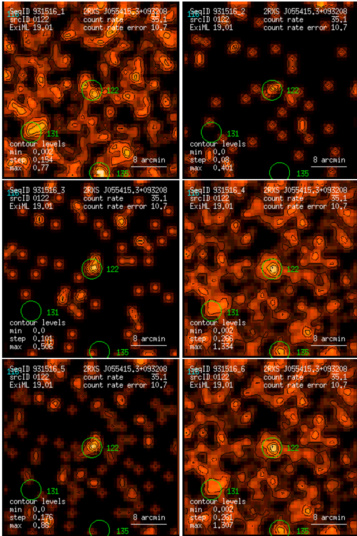
Figure 122: RASS 931516: detection 0122: band rate images, Gaussian filter: (1) PSPC channels 11 – 41, (2) 52 – 90, (3) 91 – 201, (4) 11 – 235, (5) 52 – 201, (6) 11 – 201. Broad band rates in counts/ks. Band rate contour levels in counts/ks/arcmin 2 .
