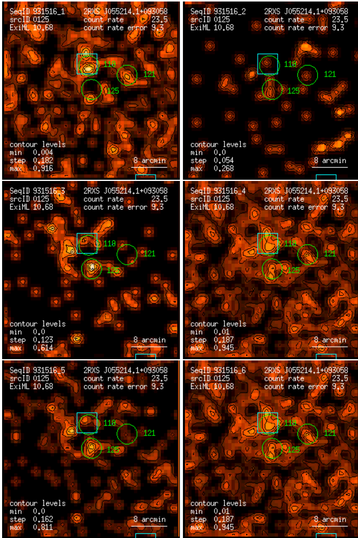
Figure 125: RASS 931516: detection 0125: band rate images, Gaussian filter: (1) PSPC channels 11 – 41, (2) 52 – 90, (3) 91 – 201, (4) 11 – 235, (5) 52 – 201, (6) 11 – 201. Broad band rates in counts/ks. Band rate contour levels in counts/ks/arcmin 2 .
