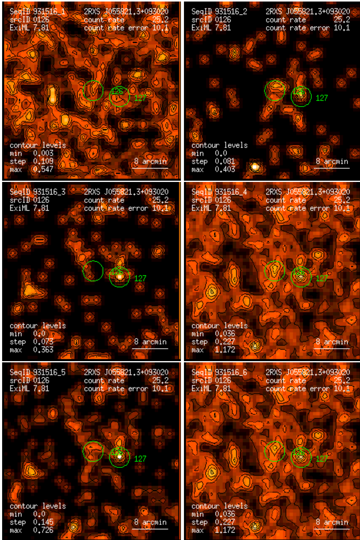
Figure 126: RASS 931516: detection 0126: band rate images, Gaussian filter: (1) PSPC channels 11 – 41, (2) 52 – 90, (3) 91 – 201, (4) 11 – 235, (5) 52 – 201, (6) 11 – 201. Broad band rates in counts/ks. Band rate contour levels in counts/ks/arcmin 2 .
