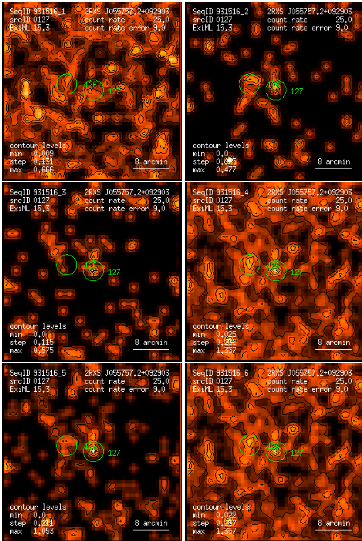
Figure 127: RASS 931516: detection 0127: band rate images, Gaussian filter: (1) PSPC channels 11 – 41, (2) 52 – 90, (3) 91 – 201, (4) 11 – 235, (5) 52 – 201, (6) 11 – 201. Broad band rates in counts/ks. Band rate contour levels in counts/ks/arcmin 2 .
