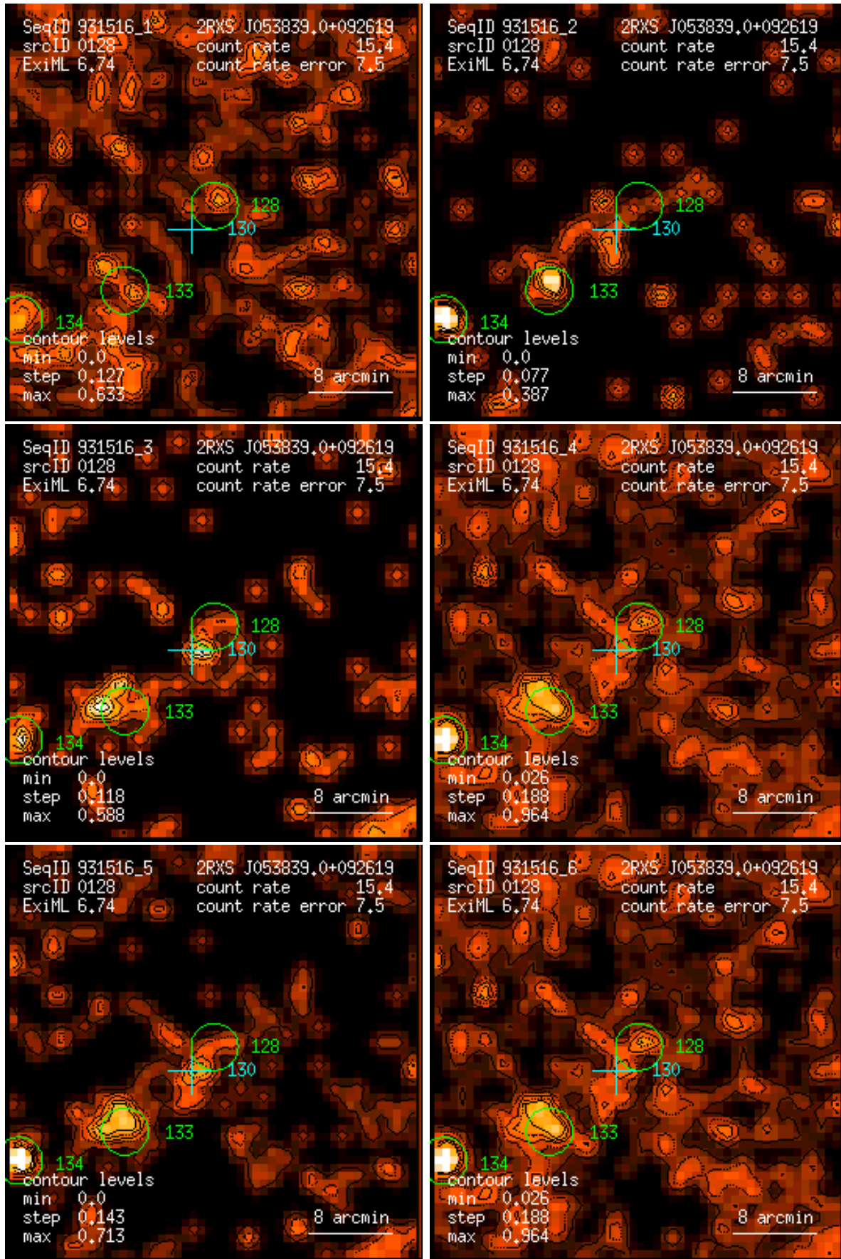
Figure 128: RASS 931516: detection 0128: band rate images, Gaussian filter: (1) PSPC channels 11 – 41, (2) 52 – 90, (3) 91 – 201, (4) 11 – 235, (5) 52 – 201, (6) 11 – 201. Broad band rates in counts/ks. Band rate contour levels in counts/ks/arcmin 2 .
