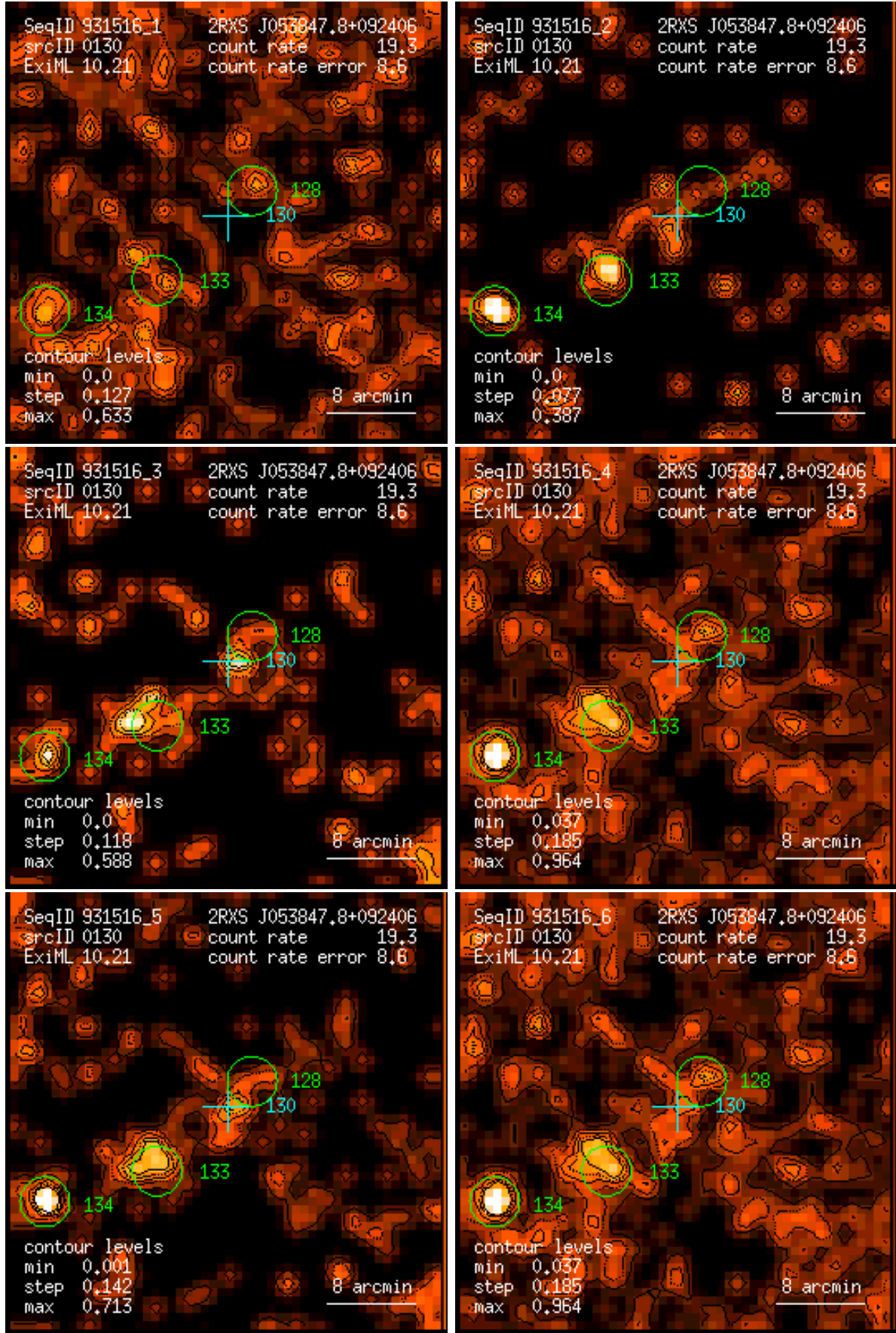
Figure 130: RASS 931516: detection 0130: band rate images, Gaussian filter: (1) PSPC channels 11 – 41, (2) 52 – 90, (3) 91 – 201, (4) 11 – 235, (5) 52 – 201, (6) 11 – 201. Broad band rates in counts/ks. Band rate contour levels in counts/ks/arcmin 2 .
