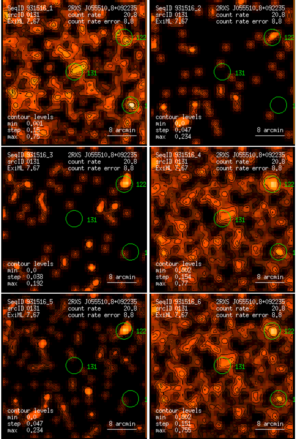
Figure 131: RASS 931516: detection 0131: band rate images, Gaussian filter: (1) PSPC channels 11 – 41, (2) 52 – 90, (3) 91 – 201, (4) 11 – 235, (5) 52 – 201, (6) 11 – 201. Broad band rates in counts/ks. Band rate contour levels in counts/ks/arcmin 2 .
