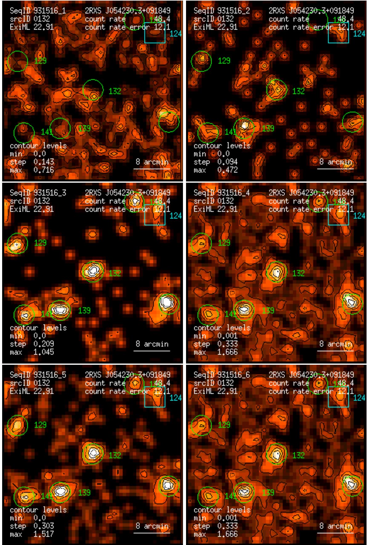
Figure 132: RASS 931516: detection 0132: band rate images, Gaussian filter: (1) PSPC channels 11 – 41, (2) 52 – 90, (3) 91 – 201, (4) 11 – 235, (5) 52 – 201, (6) 11 – 201. Broad band rates in counts/ks. Band rate contour levels in counts/ks/arcmin 2 .
