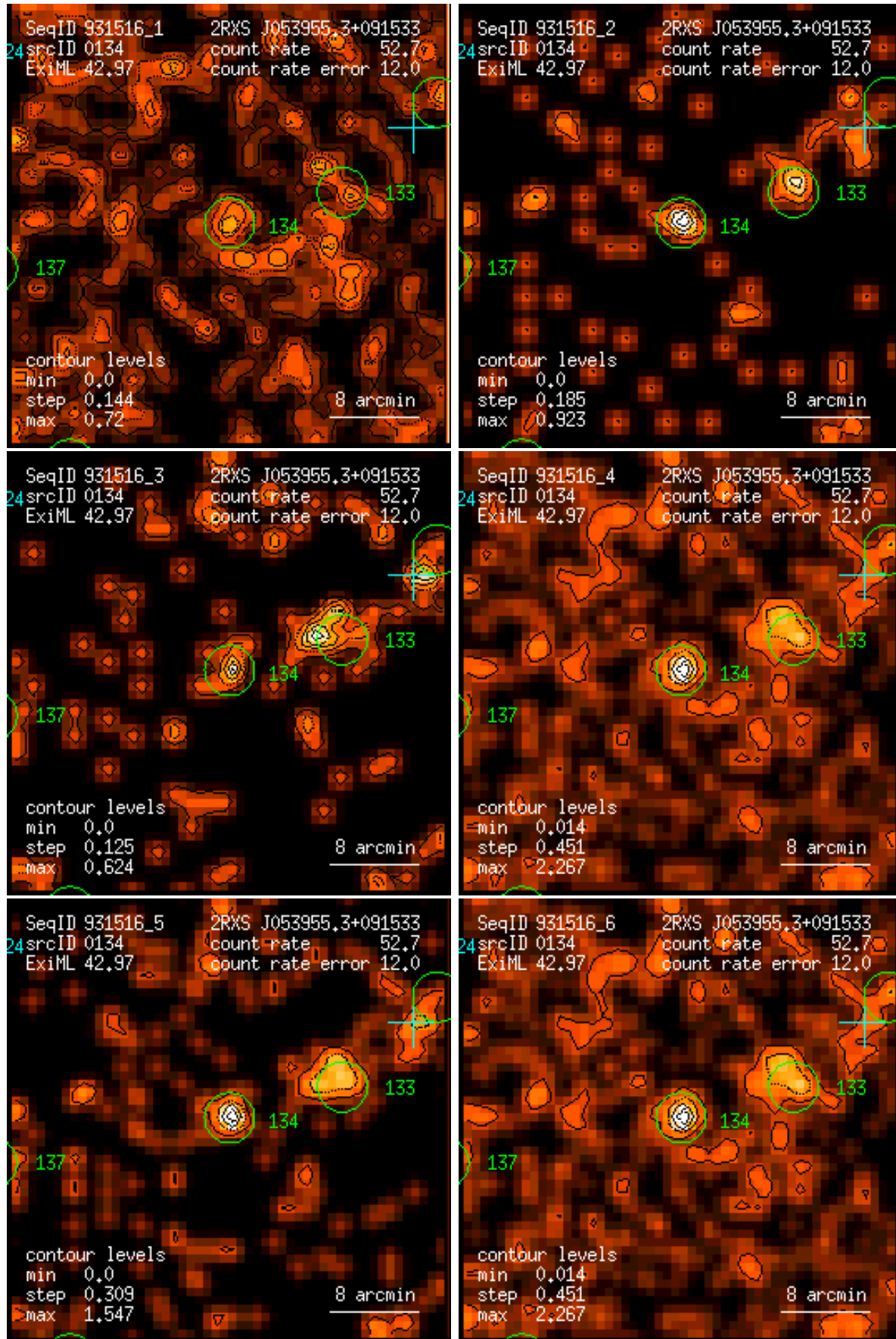
Figure 134: RASS 931516: detection 0134: band rate images, Gaussian filter: (1) PSPC channels 11 – 41, (2) 52 – 90, (3) 91 – 201, (4) 11 – 235, (5) 52 – 201, (6) 11 – 201. Broad band rates in counts/ks. Band rate contour levels in counts/ks/arcmin 2 .
