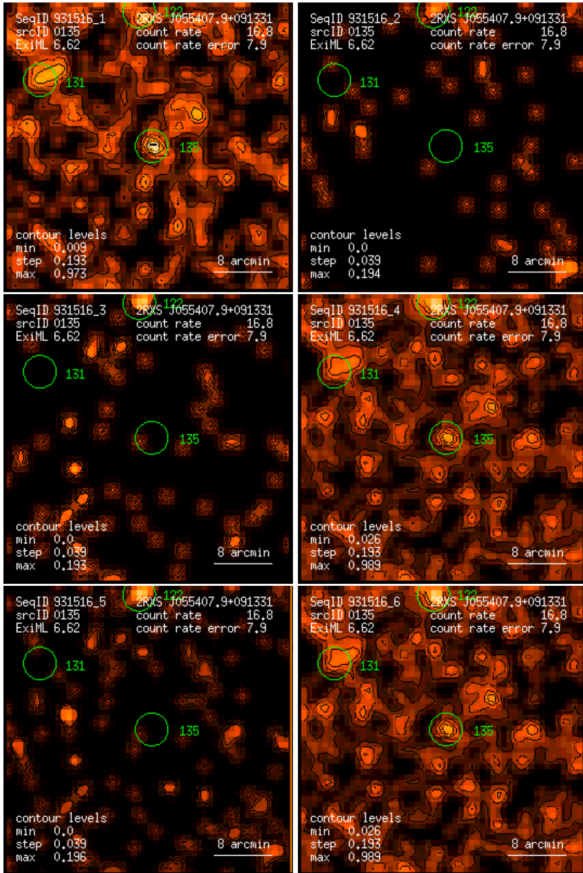
Figure 135: RASS 931516: detection 0135: band rate images, Gaussian filter: (1) PSPC channels 11 – 41, (2) 52 – 90, (3) 91 – 201, (4) 11 – 235, (5) 52 – 201, (6) 11 – 201. Broad band rates in counts/ks. Band rate contour levels in counts/ks/arcmin 2 .
