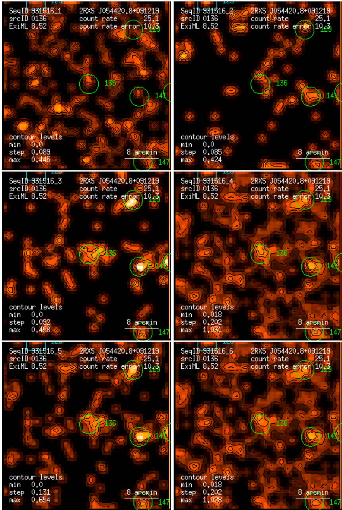
Figure 136: RASS 931516: detection 0136: band rate images, Gaussian filter: (1) PSPC channels 11 – 41, (2) 52 – 90, (3) 91 – 201, (4) 11 – 235, (5) 52 – 201, (6) 11 – 201. Broad band rates in counts/ks. Band rate contour levels in counts/ks/arcmin 2 .
