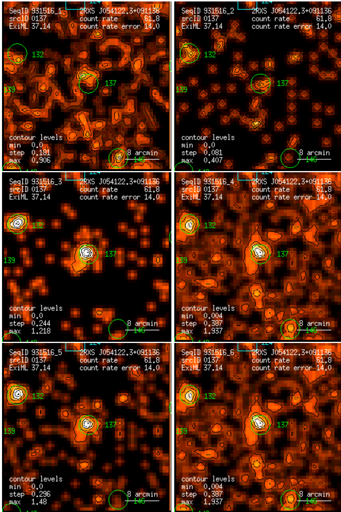
Figure 137: RASS 931516: detection 0137: band rate images, Gaussian filter: (1) PSPC channels 11 – 41, (2) 52 – 90, (3) 91 – 201, (4) 11 – 235, (5) 52 – 201, (6) 11 – 201. Broad band rates in counts/ks. Band rate contour levels in counts/ks/arcmin 2 .
