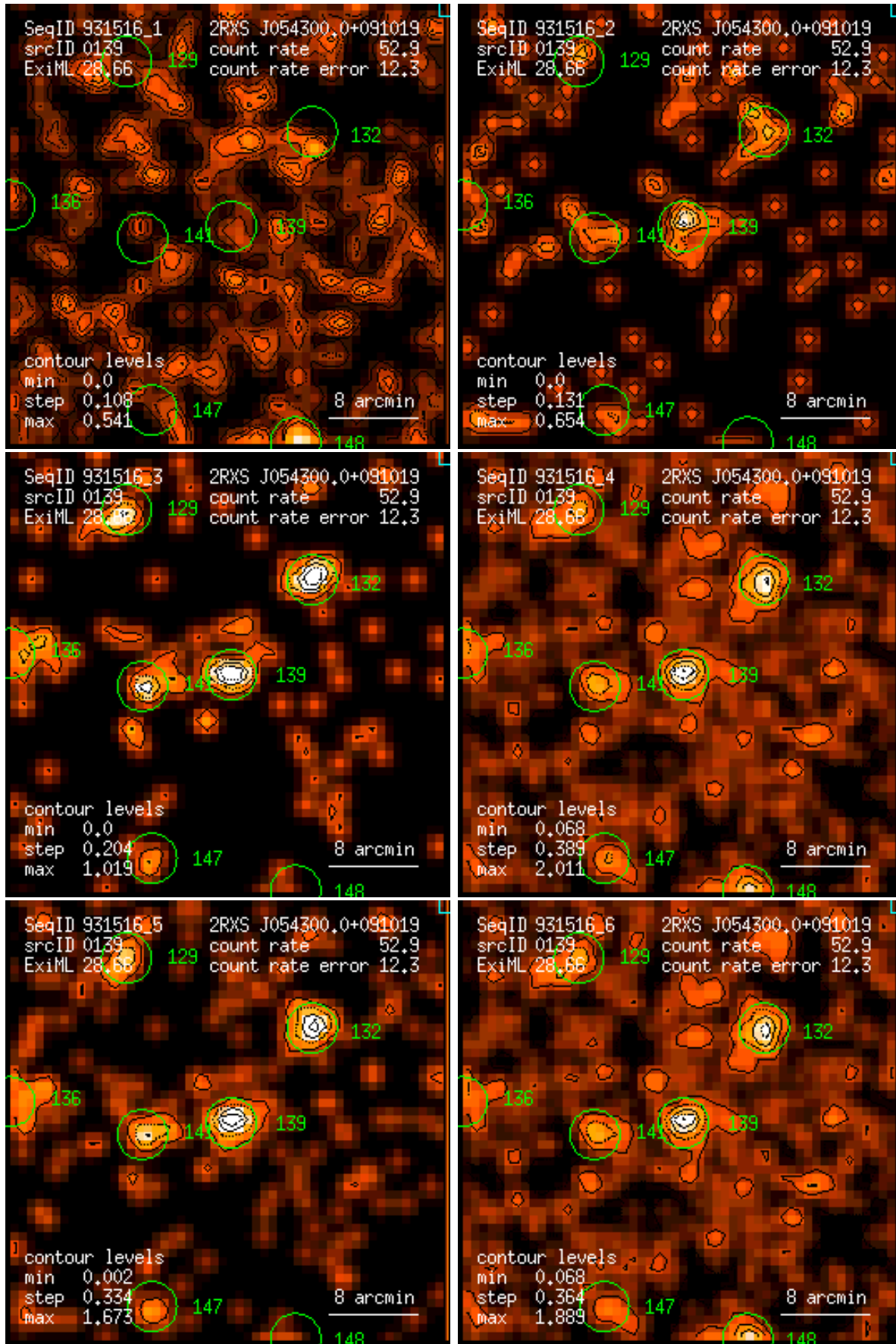
Figure 139: RASS 931516: detection 0139: band rate images, Gaussian filter: (1) PSPC channels 11 – 41, (2) 52 – 90, (3) 91 – 201, (4) 11 – 235, (5) 52 – 201, (6) 11 – 201. Broad band rates in counts/ks. Band rate contour levels in counts/ks/arcmin 2 .
