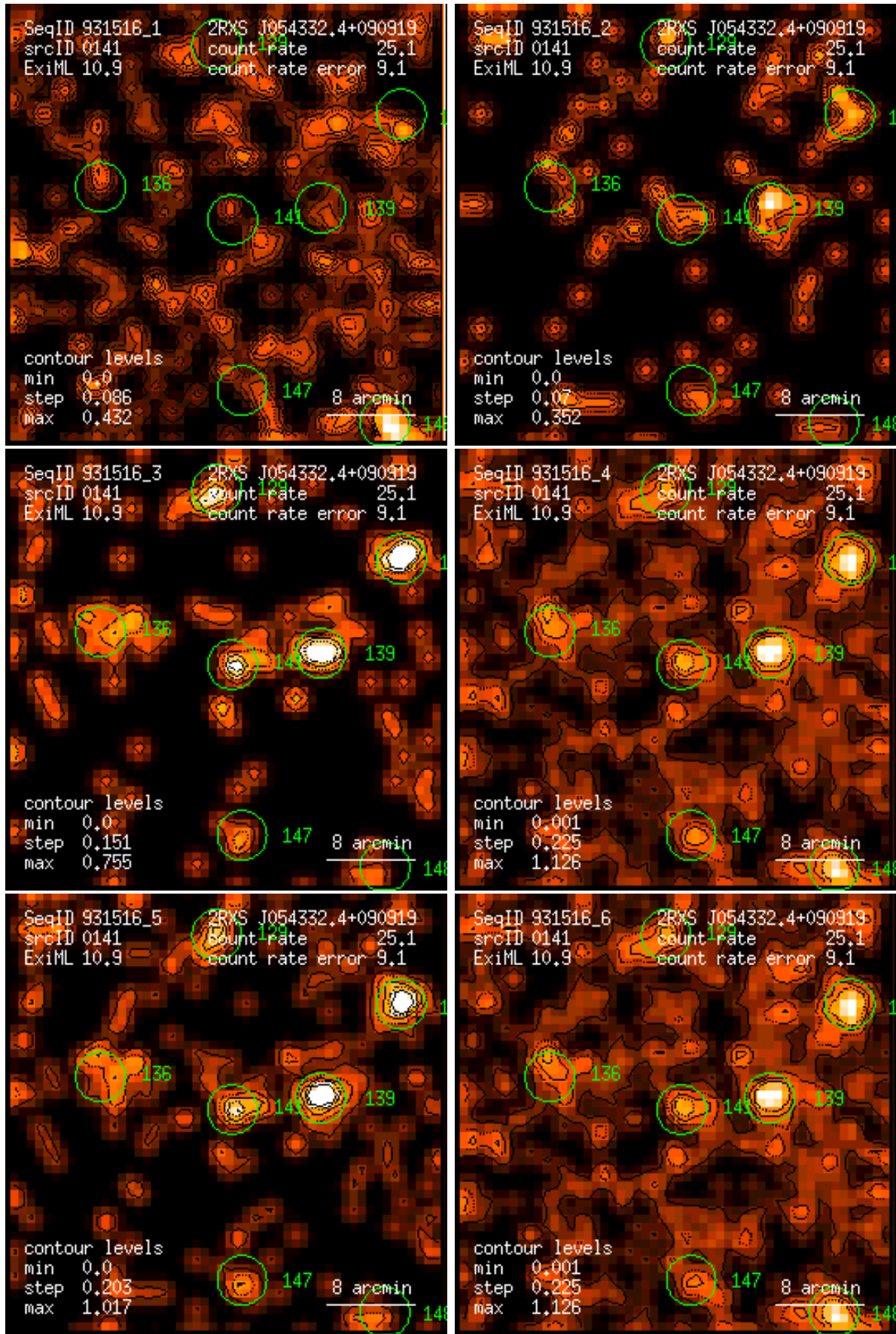
Figure 141: RASS 931516: detection 0141: band rate images, Gaussian filter: (1) PSPC channels 11 – 41, (2) 52 – 90, (3) 91 – 201, (4) 11 – 235, (5) 52 – 201, (6) 11 – 201. Broad band rates in counts/ks. Band rate contour levels in counts/ks/arcmin 2 .
