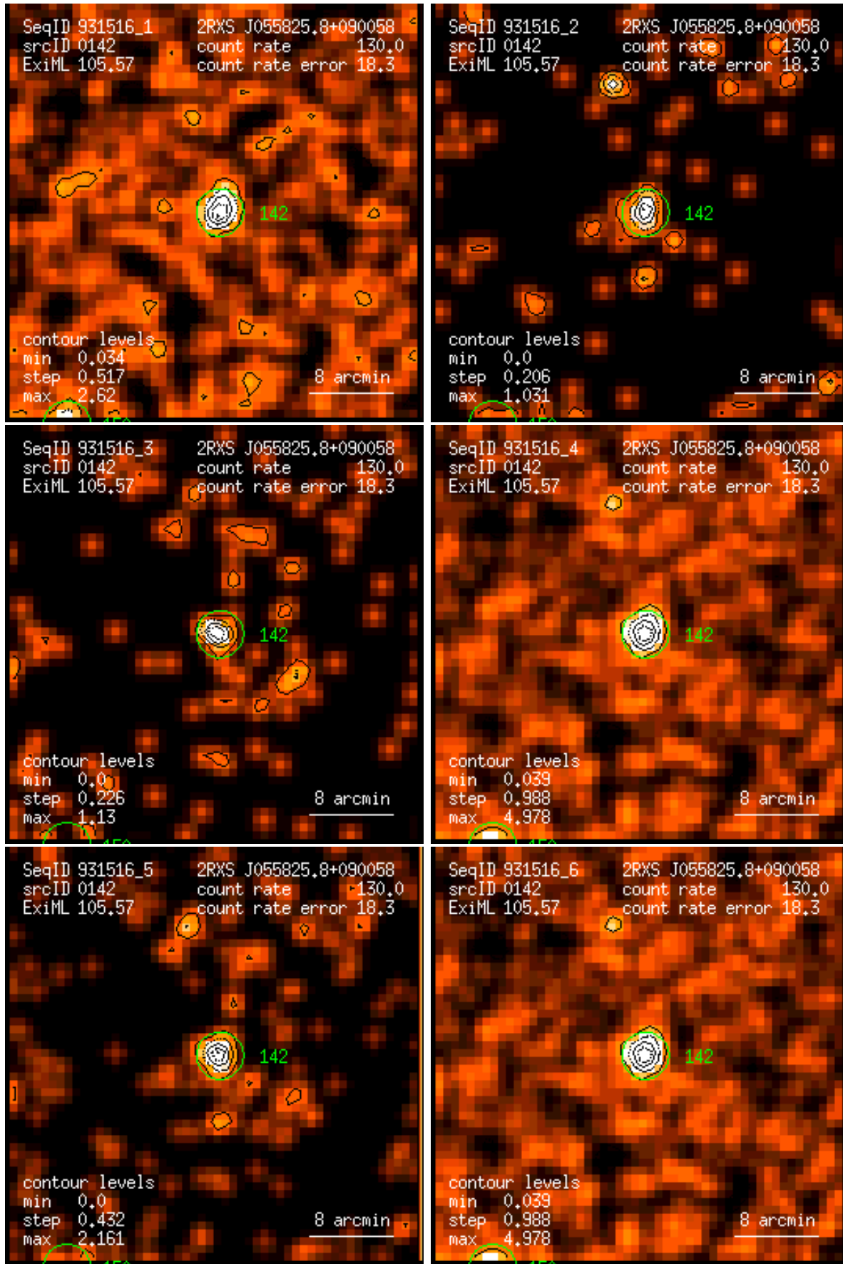
Figure 142: RASS 931516: detection 0142: band rate images, Gaussian filter: (1) PSPC channels 11 – 41, (2) 52 – 90, (3) 91 – 201, (4) 11 – 235, (5) 52 – 201, (6) 11 – 201. Broad band rates in counts/ks. Band rate contour levels in counts/ks/arcmin 2 .
