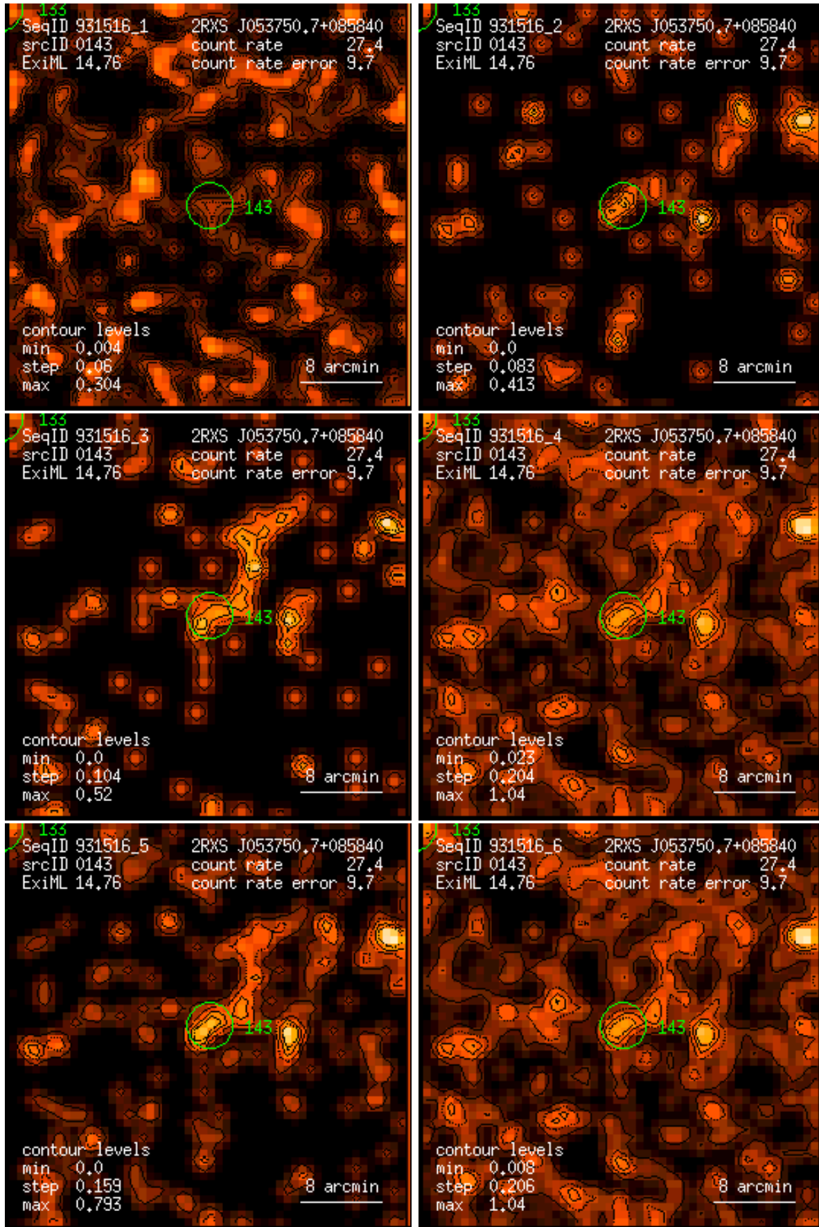
Figure 143: RASS 931516: detection 0143: band rate images, Gaussian filter: (1) PSPC channels 11 – 41, (2) 52 – 90, (3) 91 – 201, (4) 11 – 235, (5) 52 – 201, (6) 11 – 201. Broad band rates in counts/ks. Band rate contour levels in counts/ks/arcmin 2 .
