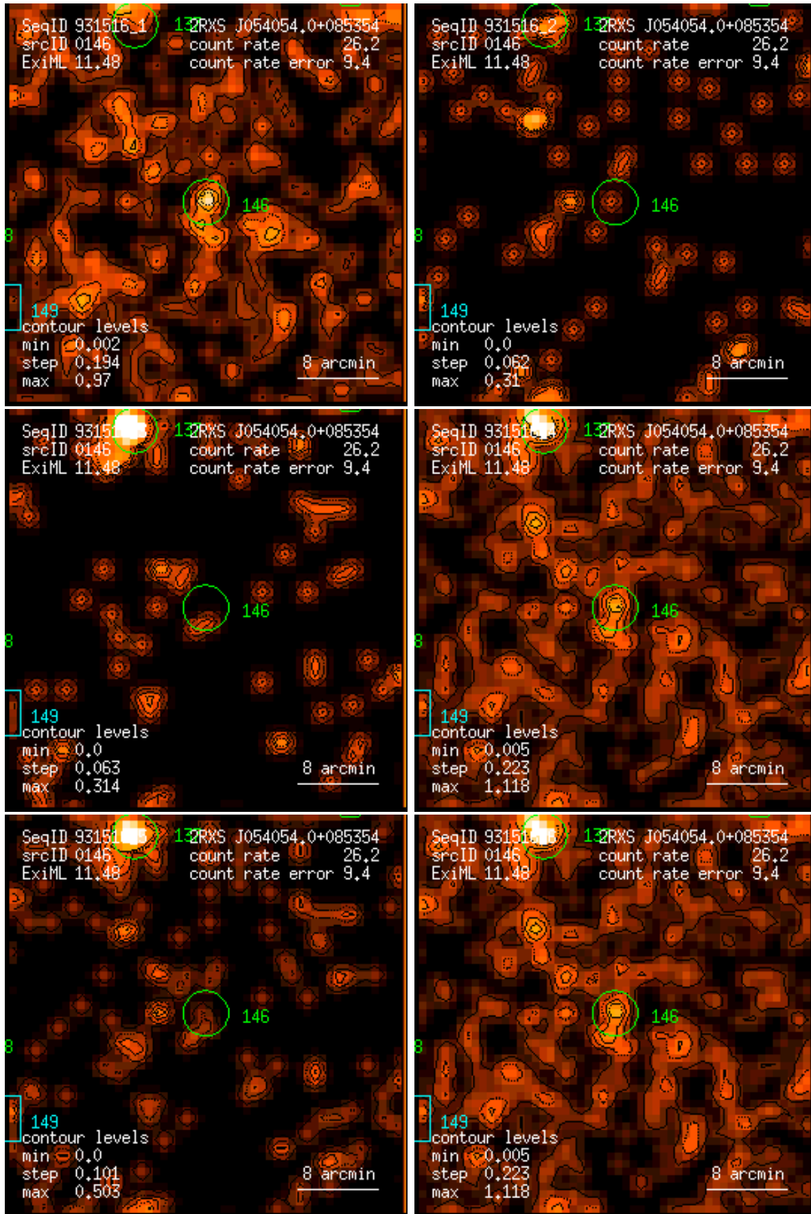
Figure 146: RASS 931516: detection 0146: band rate images, Gaussian filter: (1) PSPC channels 11 – 41, (2) 52 – 90, (3) 91 – 201, (4) 11 – 235, (5) 52 – 201, (6) 11 – 201. Broad band rates in counts/ks. Band rate contour levels in counts/ks/arcmin 2 .
