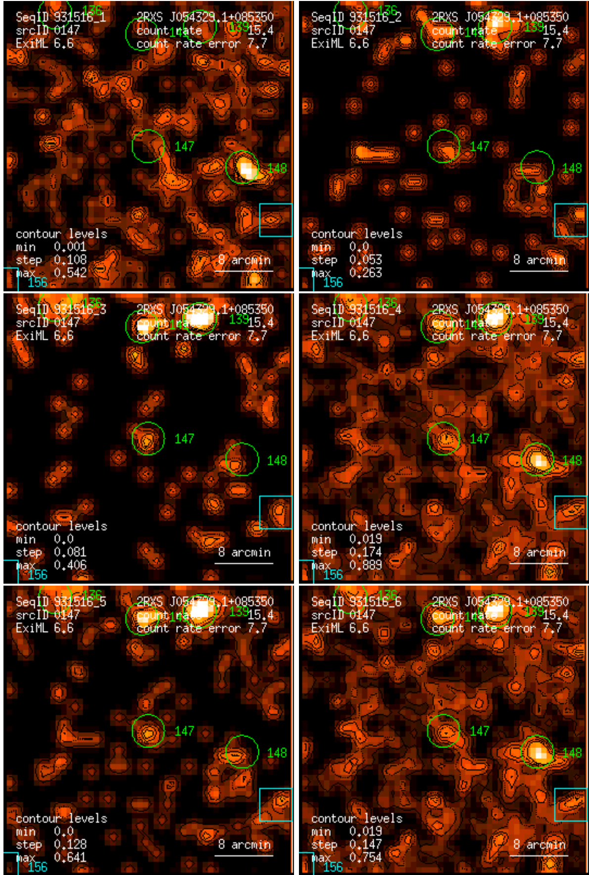
Figure 147: RASS 931516: detection 0147: band rate images, Gaussian filter: (1) PSPC channels 11 – 41, (2) 52 – 90, (3) 91 – 201, (4) 11 – 235, (5) 52 – 201, (6) 11 – 201. Broad band rates in counts/ks. Band rate contour levels in counts/ks/arcmin 2 .
