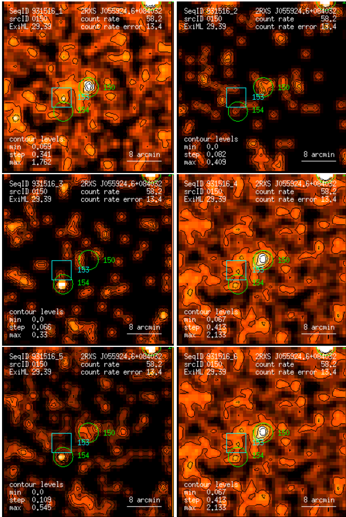
Figure 150: RASS 931516: detection 0150: band rate images, Gaussian filter: (1) PSPC channels 11 – 41, (2) 52 – 90, (3) 91 – 201, (4) 11 – 235, (5) 52 – 201, (6) 11 – 201. Broad band rates in counts/ks. Band rate contour levels in counts/ks/arcmin 2 .
