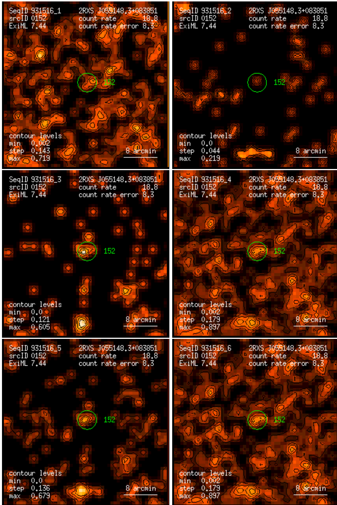
Figure 152: RASS 931516: detection 0152: band rate images, Gaussian filter: (1) PSPC channels 11 – 41, (2) 52 – 90, (3) 91 – 201, (4) 11 – 235, (5) 52 – 201, (6) 11 – 201. Broad band rates in counts/ks. Band rate contour levels in counts/ks/arcmin 2 .
