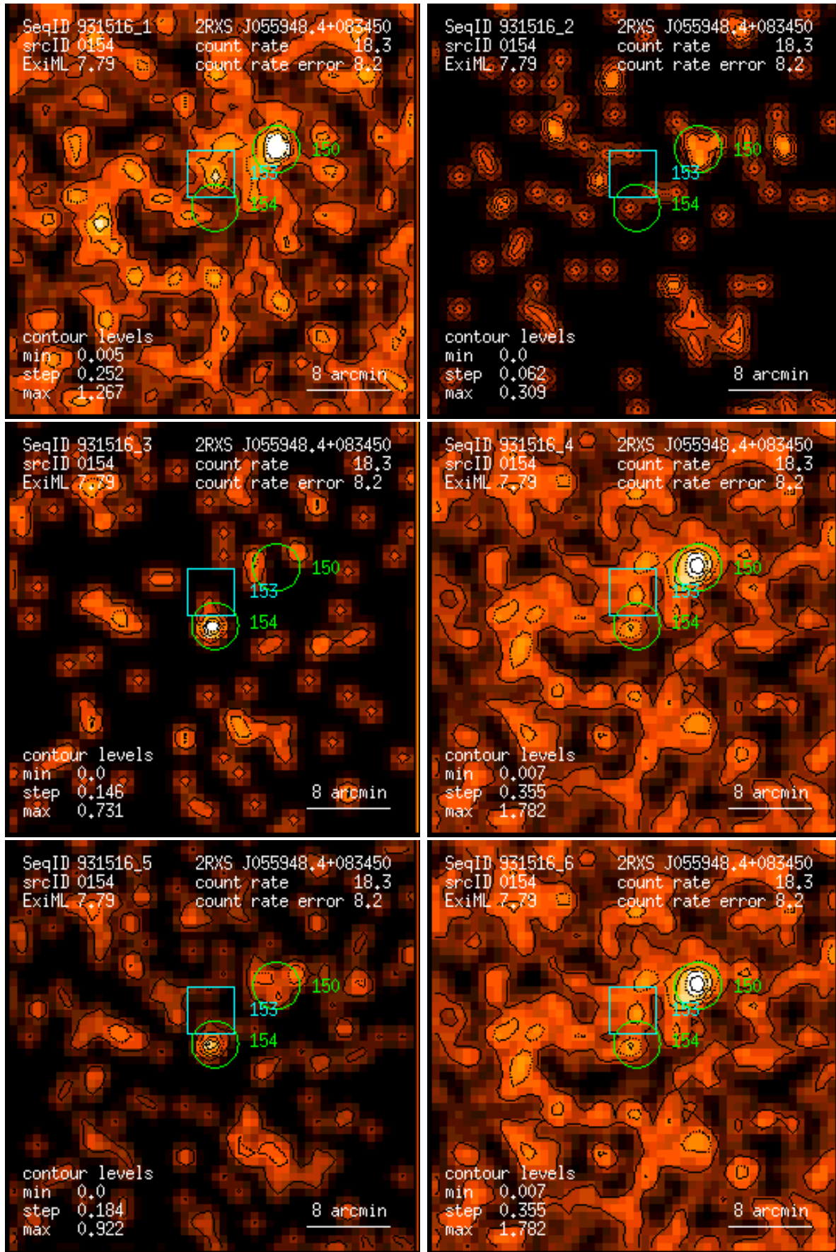
Figure 154: RASS 931516: detection 0154: band rate images, Gaussian filter: (1) PSPC channels 11 – 41, (2) 52 – 90, (3) 91 – 201, (4) 11 – 235, (5) 52 – 201, (6) 11 – 201. Broad band rates in counts/ks. Band rate contour levels in counts/ks/arcmin 2 .
