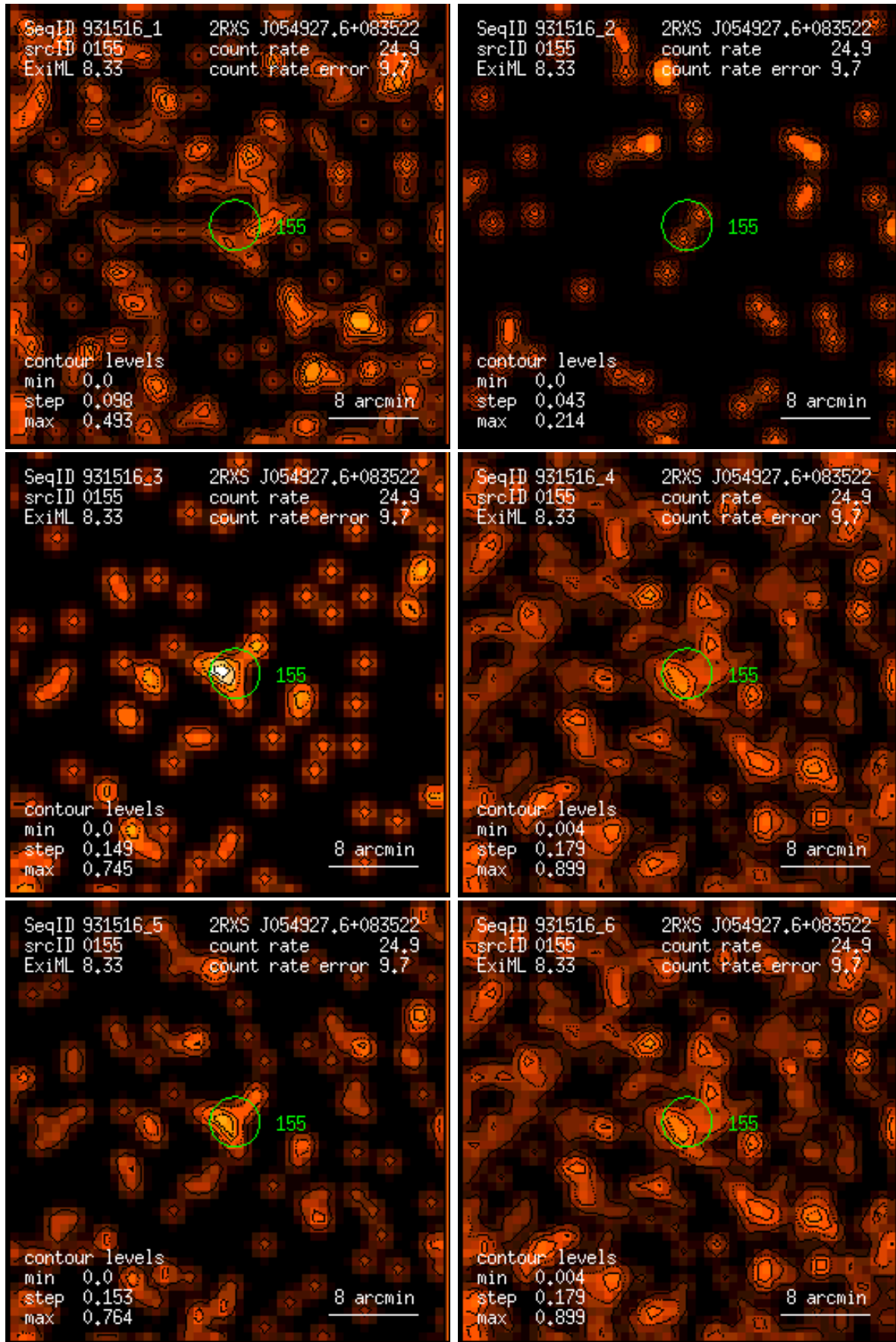
Figure 155: RASS 931516: detection 0155: band rate images, Gaussian filter: (1) PSPC channels 11 – 41, (2) 52 – 90, (3) 91 – 201, (4) 11 – 235, (5) 52 – 201, (6) 11 – 201. Broad band rates in counts/ks. Band rate contour levels in counts/ks/arcmin 2 .
