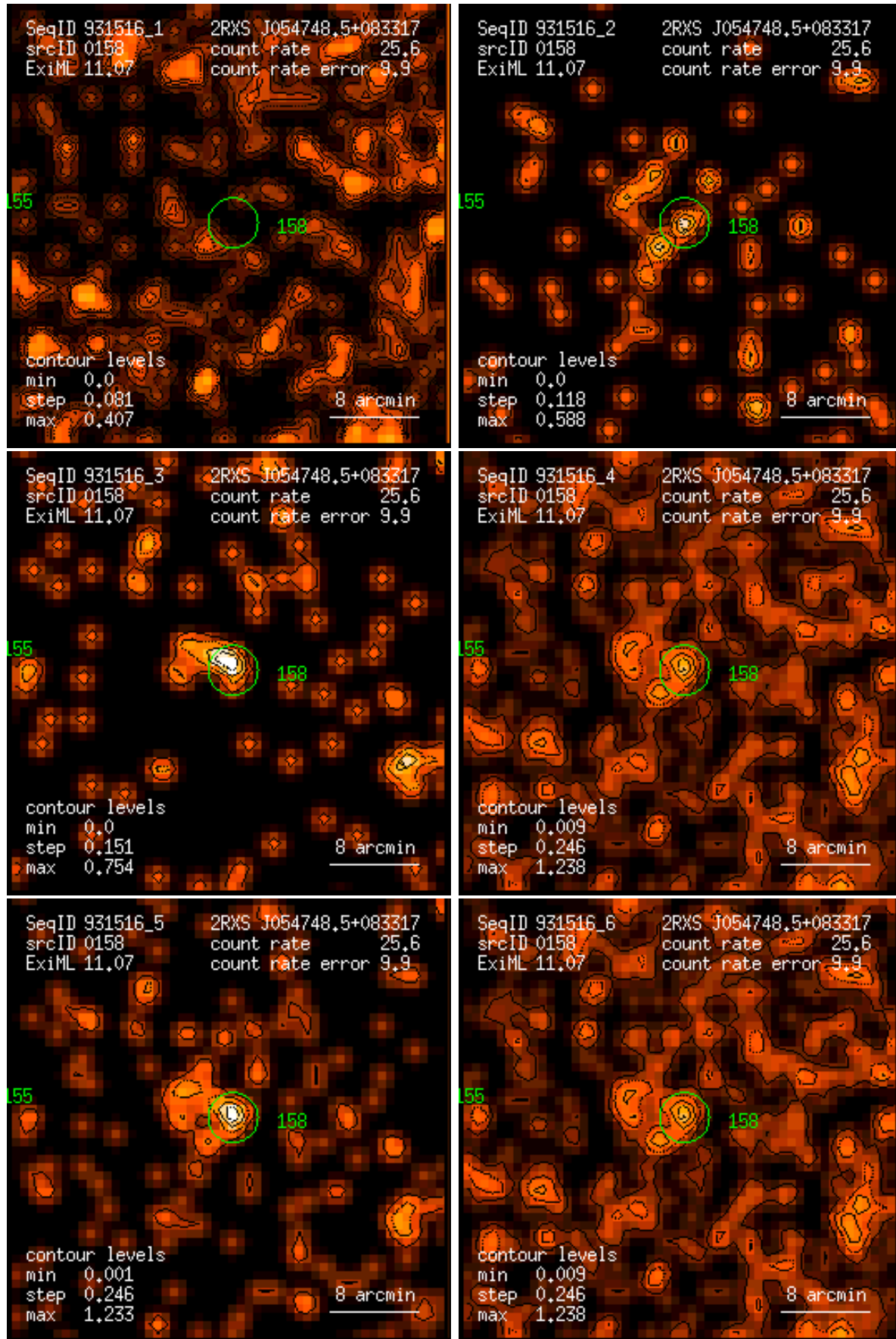
Figure 158: RASS 931516: detection 0158: band rate images, Gaussian filter: (1) PSPC channels 11 – 41, (2) 52 – 90, (3) 91 – 201, (4) 11 – 235, (5) 52 – 201, (6) 11 – 201. Broad band rates in counts/ks. Band rate contour levels in counts/ks/arcmin 2 .
