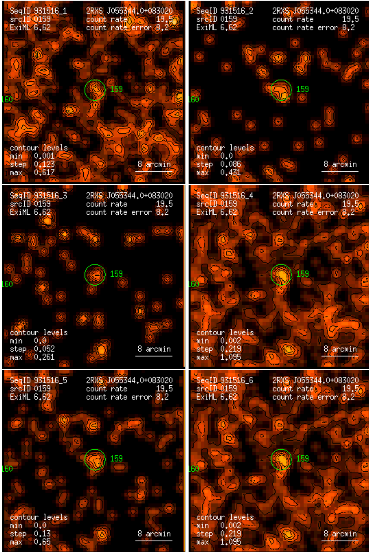
Figure 159: RASS 931516: detection 0159: band rate images, Gaussian filter: (1) PSPC channels 11 – 41, (2) 52 – 90, (3) 91 – 201, (4) 11 – 235, (5) 52 – 201, (6) 11 – 201. Broad band rates in counts/ks. Band rate contour levels in counts/ks/arcmin 2 .
