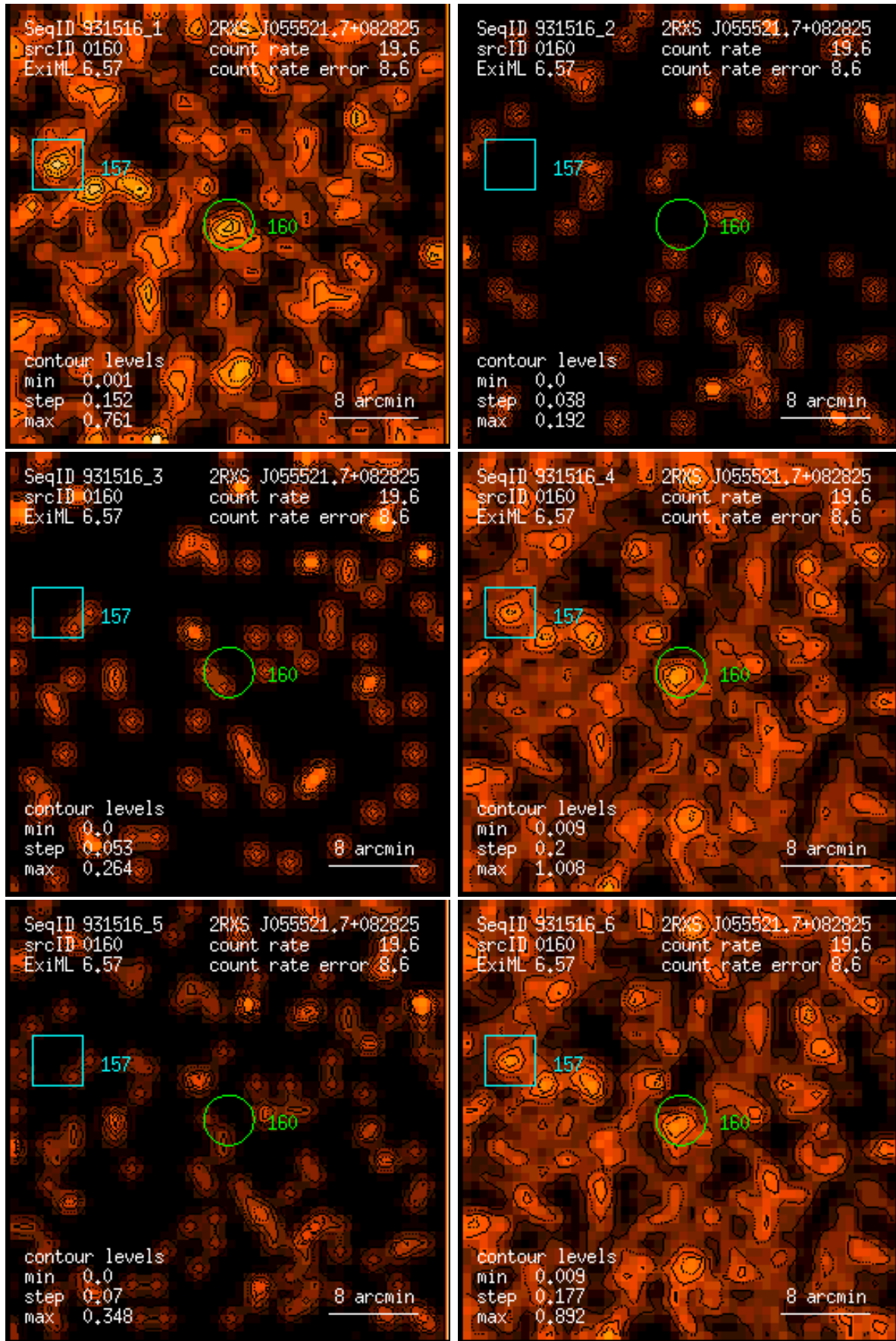
Figure 160: RASS 931516: detection 0160: band rate images, Gaussian filter: (1) PSPC channels 11 – 41, (2) 52 – 90, (3) 91 – 201, (4) 11 – 235, (5) 52 – 201, (6) 11 – 201. Broad band rates in counts/ks. Band rate contour levels in counts/ks/arcmin 2 .
