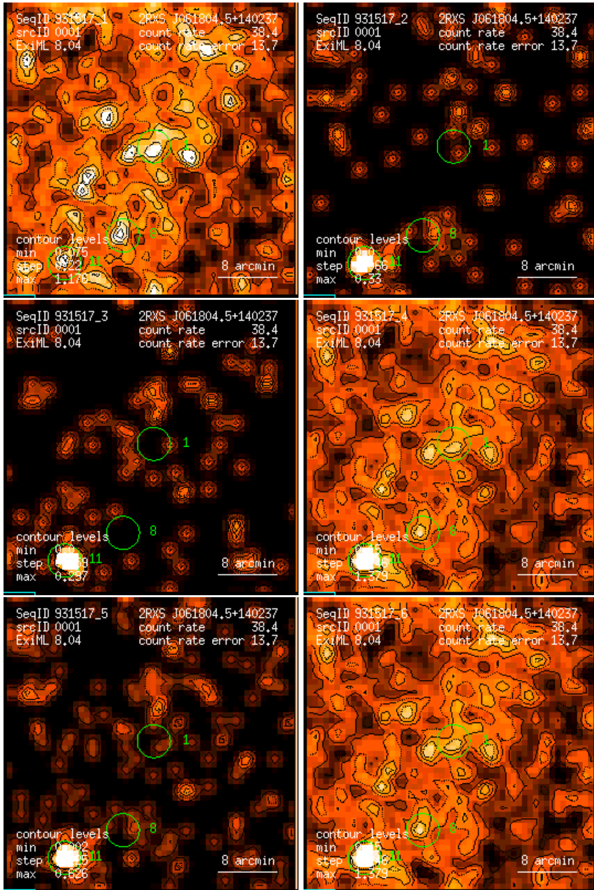
Figure 1: RASS 931517: detection 0001: band rate images, Gaussian filter: (1) PSPC channels 11 – 41, (2) 52 – 90, (3) 91 – 201, (4) 11 – 235, (5) 52 – 201, (6) 11 – 201. Broad band rates in counts/ks. Band rate contour levels in counts/ks/arcmin 2 .
