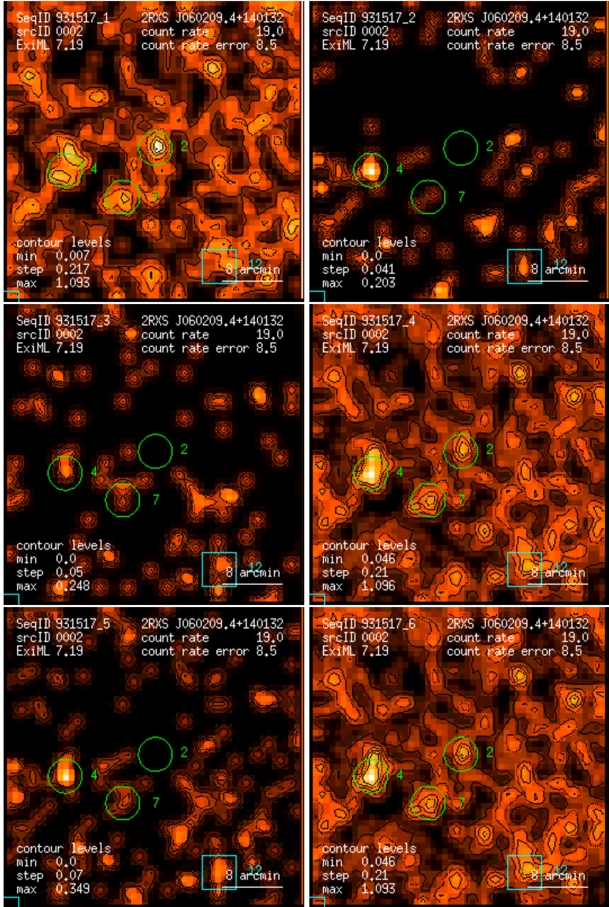
Figure 2: RASS 931517: detection 0002: band rate images, Gaussian filter: (1) PSPC channels 11 – 41, (2) 52 – 90, (3) 91 – 201, (4) 11 – 235, (5) 52 – 201, (6) 11 – 201. Broad band rates in counts/ks. Band rate contour levels in counts/ks/arcmin 2 .
