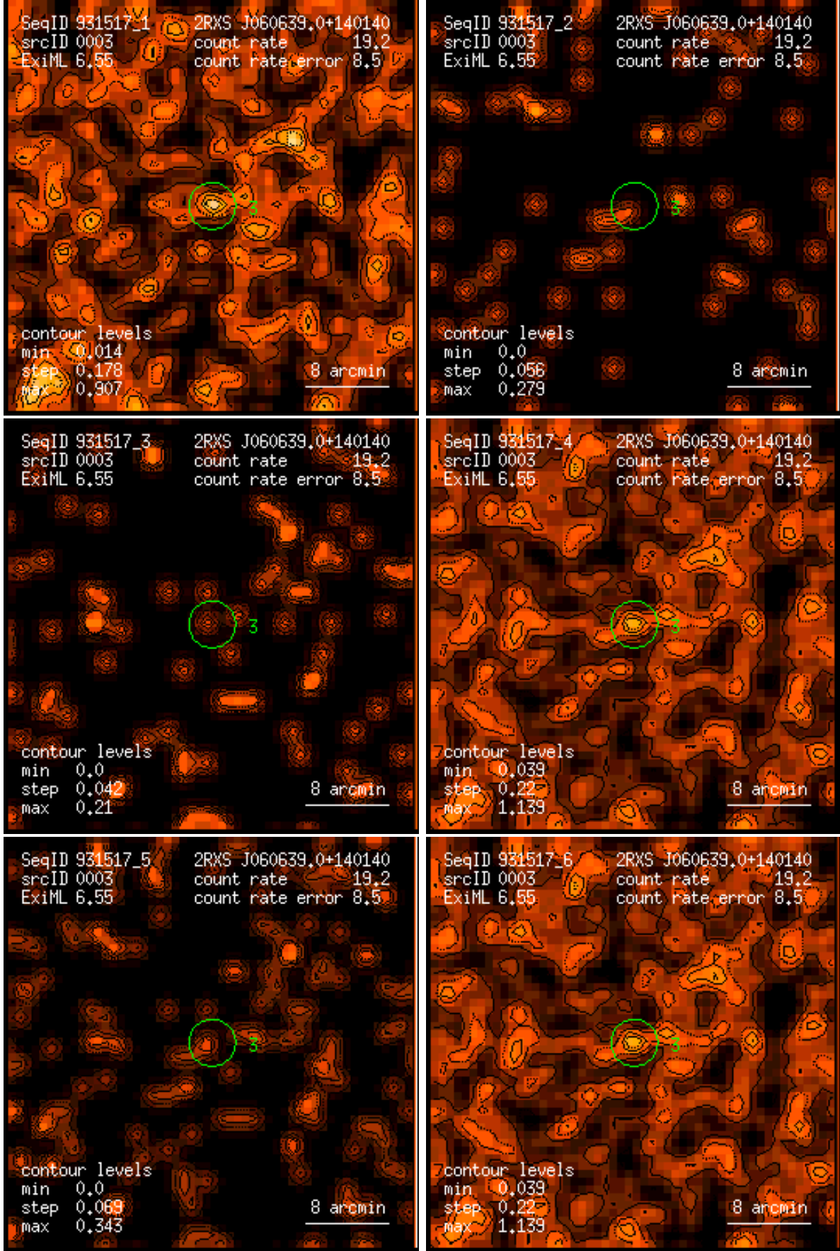
Figure 3: RASS 931517: detection 0003: band rate images, Gaussian filter: (1) PSPC channels 11 – 41, (2) 52 – 90, (3) 91 – 201, (4) 11 – 235, (5) 52 – 201, (6) 11 – 201. Broad band rates in counts/ks. Band rate contour levels in counts/ks/arcmin 2 .
