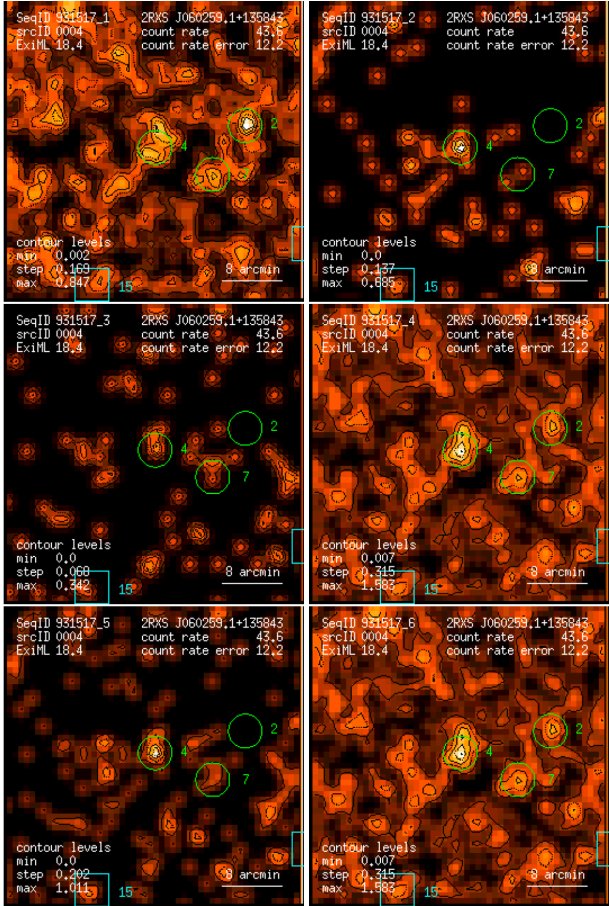
Figure 4: RASS 931517: detection 0004: band rate images, Gaussian filter: (1) PSPC channels 11 – 41, (2) 52 – 90, (3) 91 – 201, (4) 11 – 235, (5) 52 – 201, (6) 11 – 201. Broad band rates in counts/ks. Band rate contour levels in counts/ks/arcmin 2 .
