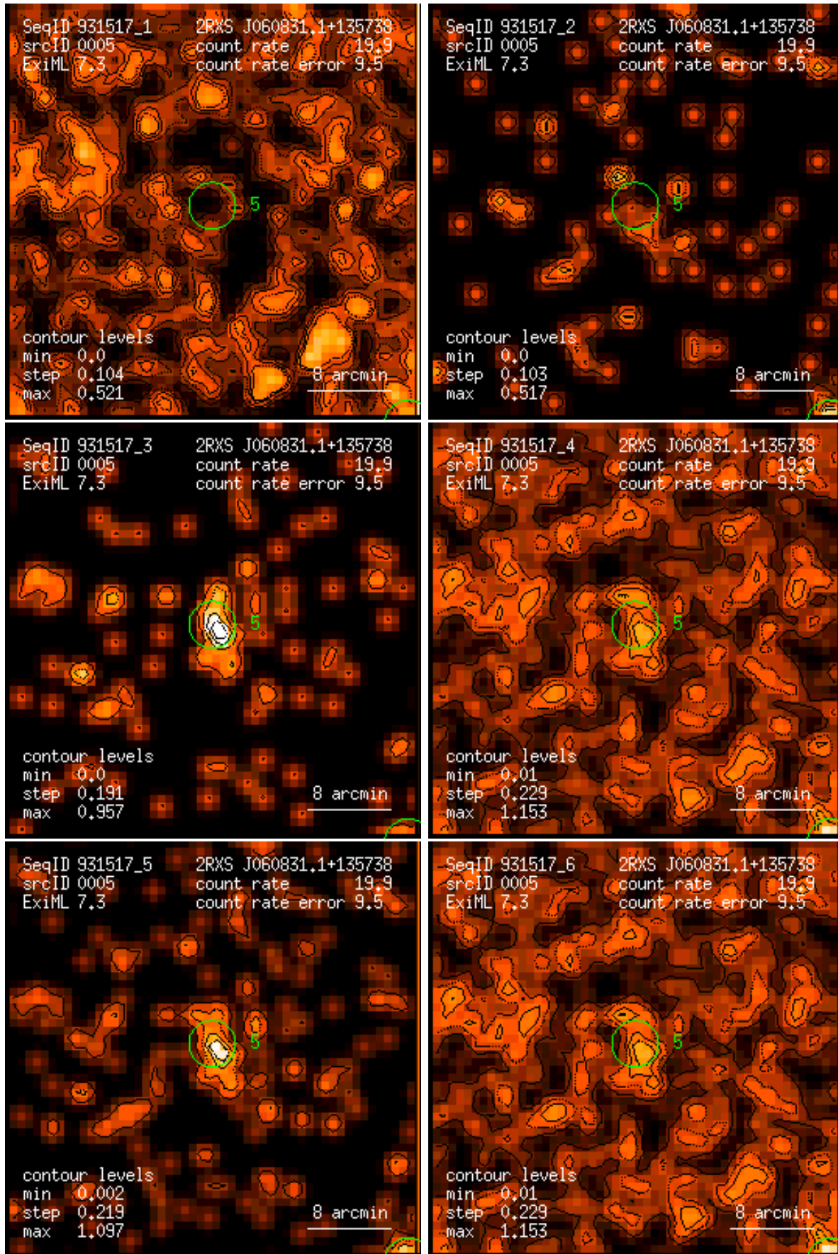
Figure 5: RASS 931517: detection 0005: band rate images, Gaussian filter: (1) PSPC channels 11 – 41, (2) 52 – 90, (3) 91 – 201, (4) 11 – 235, (5) 52 – 201, (6) 11 – 201. Broad band rates in counts/ks. Band rate contour levels in counts/ks/arcmin 2 .
